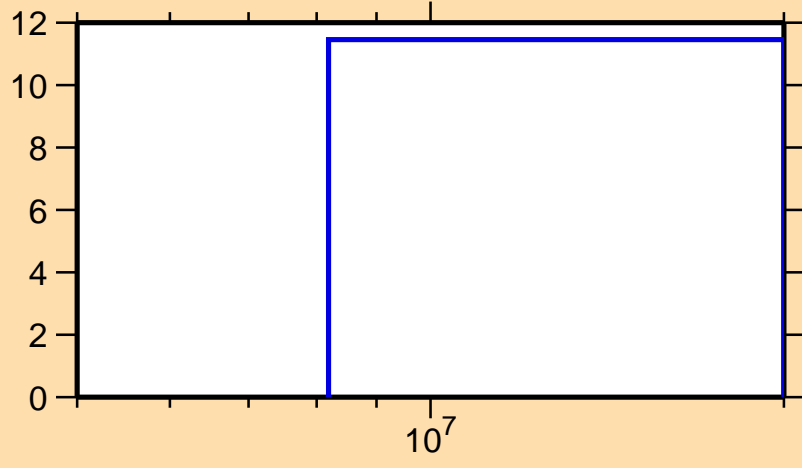
\Delta\sigma/\sigma vs. E for ^{134}\text{Sm}(n,\text{el.})
