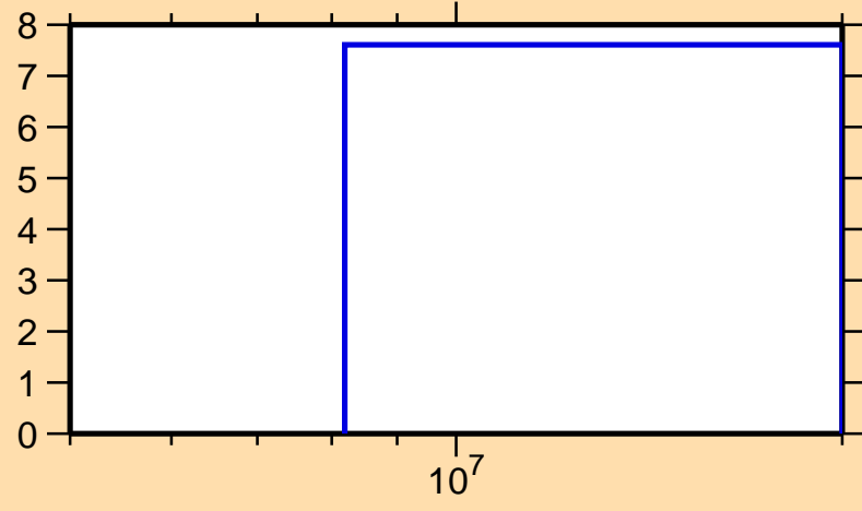
\Delta\sigma/\sigma vs. E for ^{134}\text{Sm}(n,\text{tot.})
