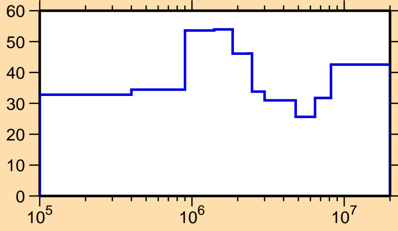
\Delta\sigma/\sigma vs. E for ^{134}\text{Sm}(n,n_1)
