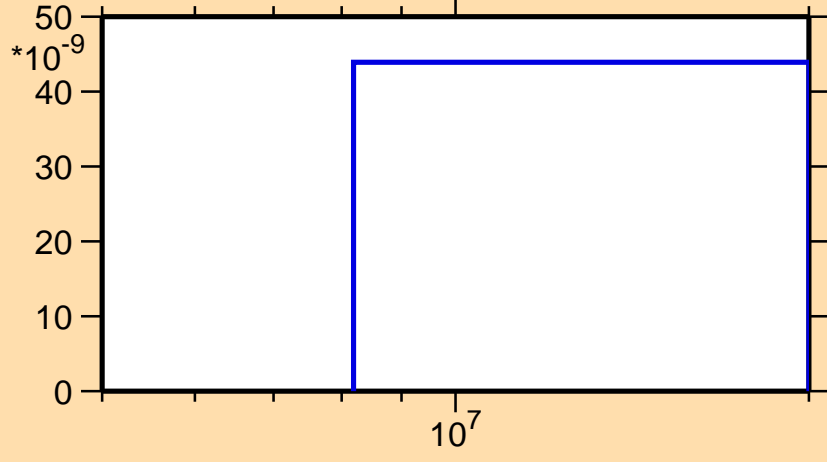
\sigma vs. E for ^{134}\text{Sm}(n,\text{pt})
