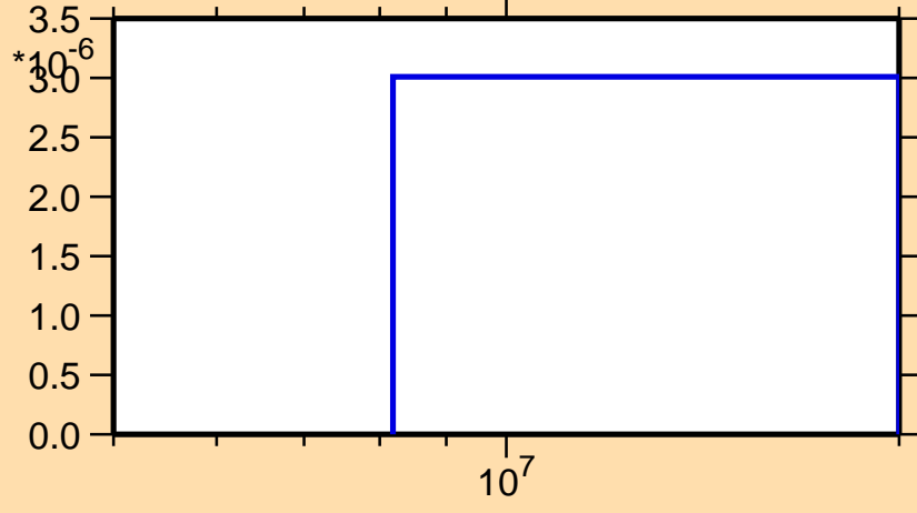
\sigma vs. E for ^{134}\text{Sm} (mt 45)
