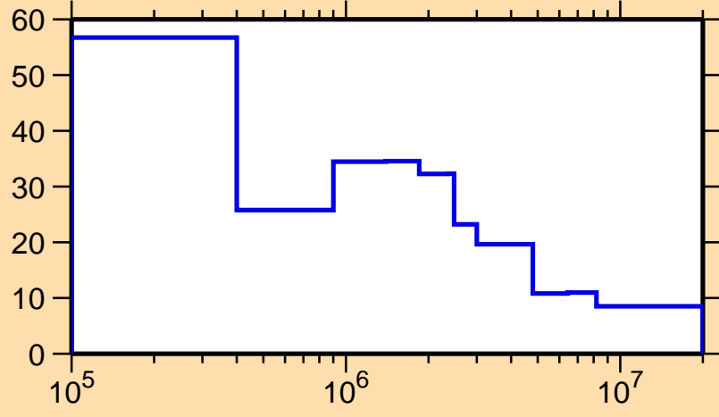
\Delta\sigma/\sigma vs. E for ^{134}\text{Sm}(n,\text{nonel.})
