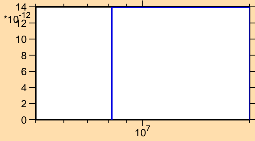
\sigma vs. E for ^{134}\text{Sm} (mt 34)
