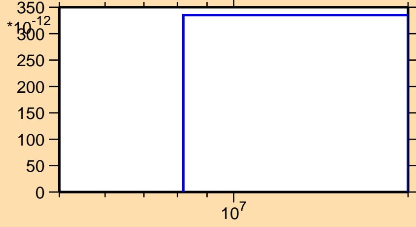
\sigma vs. E for ^{134}\text{Sm}(n,\text{nd})
