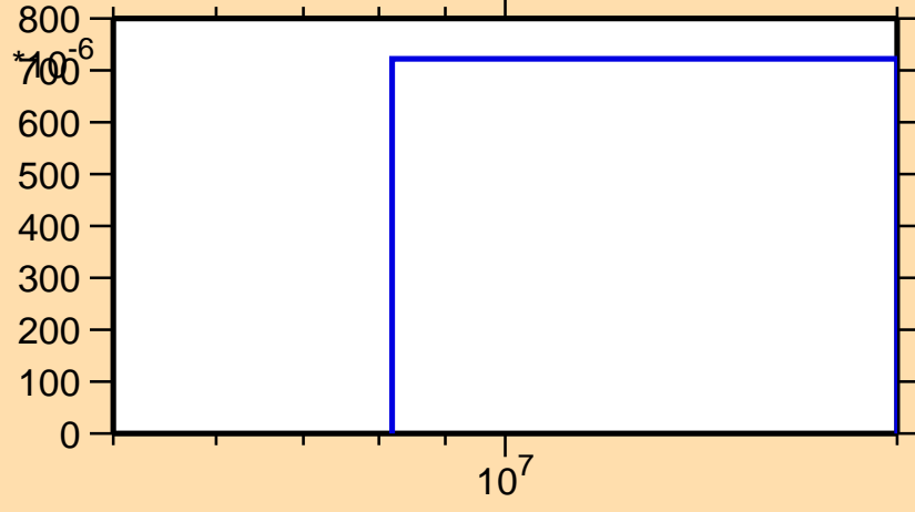
\sigma vs. E for ^{134}\text{Sm}(n,2n)
