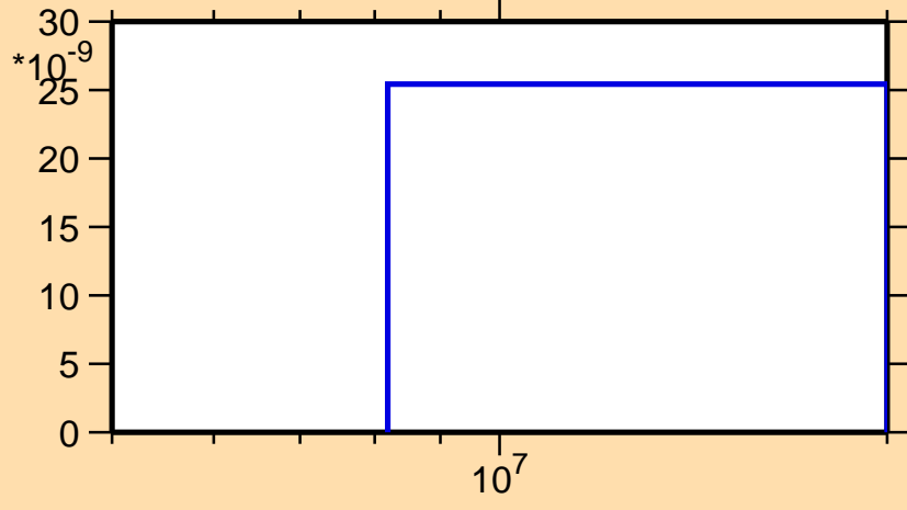
\sigma vs. E for ^{134}\text{Sm}(n,2np)
