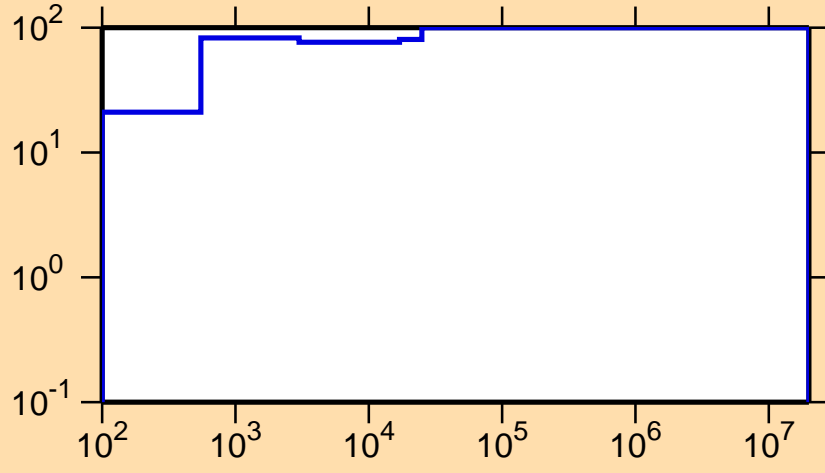
\Delta\sigma/\sigma vs. E for ^{134}\text{Sm}(n,\gamma)
