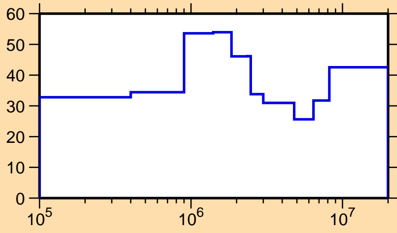
\Delta\sigma/\sigma vs. E for ^{134}\text{Sm}(n,n_1)
