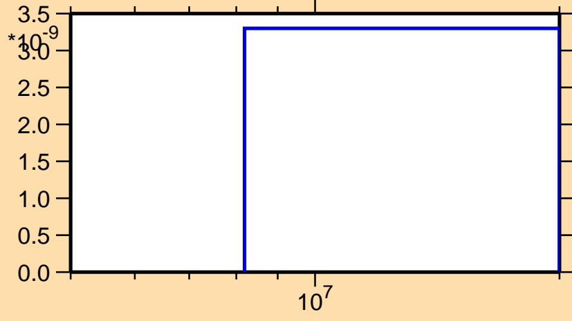
\sigma vs. E for ^{134}\text{Sm}(n,2n\alpha)
