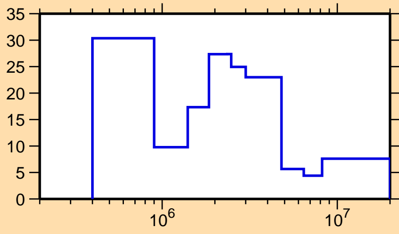
\Delta\sigma/\sigma vs. E for ^{134}\text{Sm}(n, \text{tot.})
