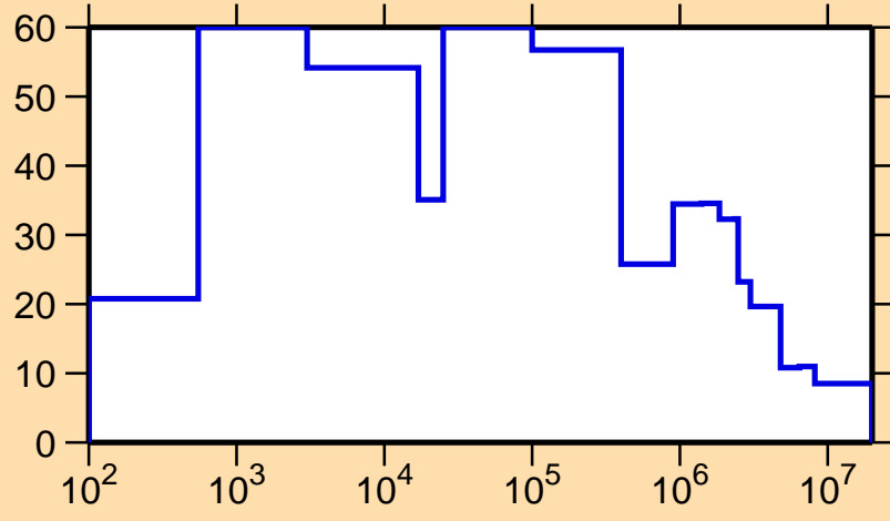
\Delta\sigma/\sigma vs. E for ^{134}\text{Sm}(n,\text{nonel.})
