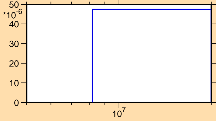
\sigma vs. E for ^{134}\text{Sm}(n,t)
