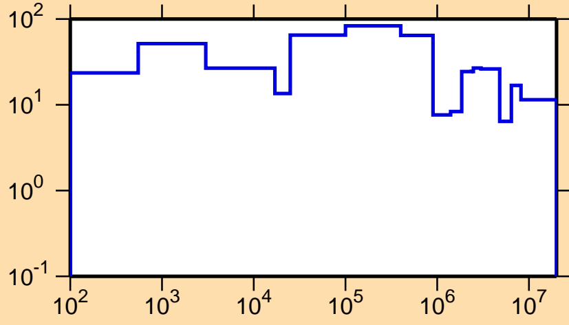
\Delta\sigma/\sigma vs. E for ^{134}\text{Sm}(n,el.)
