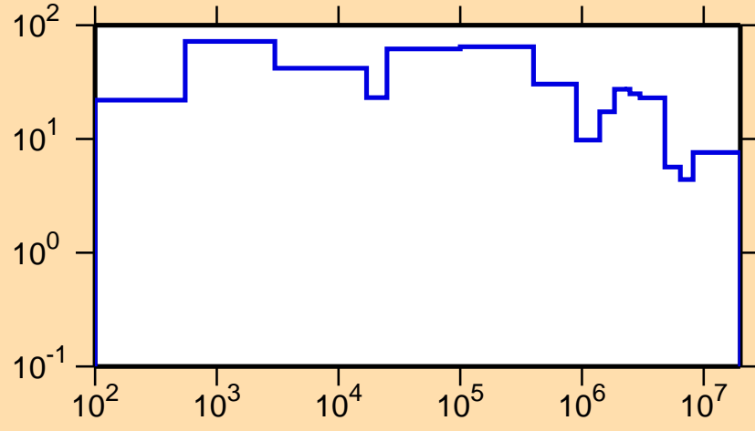
\Delta\sigma/\sigma vs. E for ^{134}\text{Sm}(n,\text{tot.})
