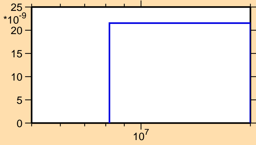
\sigma vs. E for ^{134}\text{Sm}(\text{mt117})
