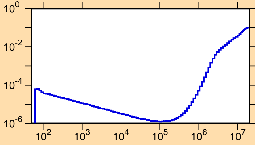
\sigma vs. E for ^{135}\text{Sm}(n,p\alpha)
