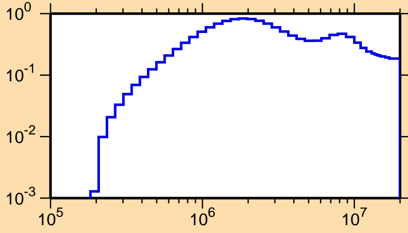
\sigma vs. E for ^{135}\text{Sm}(n,\text{inel.})
