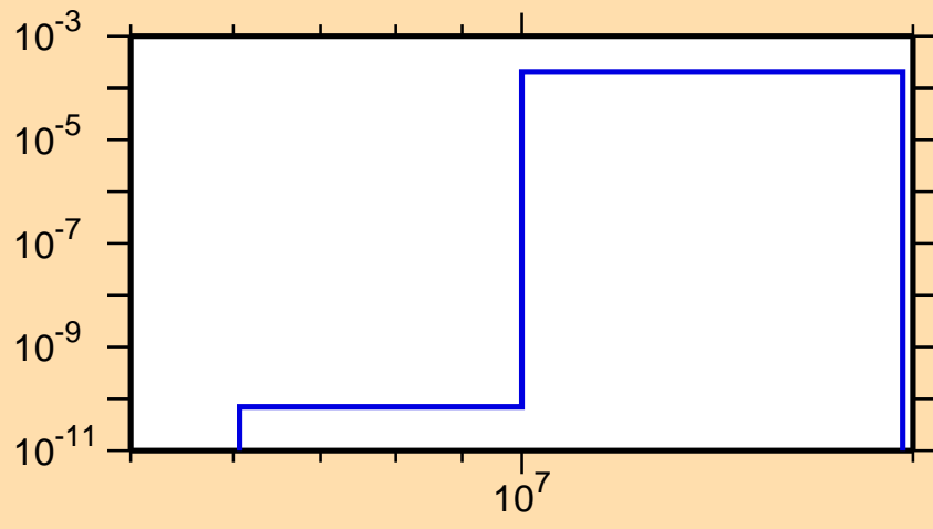
\sigma vs. E for ^{135}\text{Sm}(n,\text{pd})
