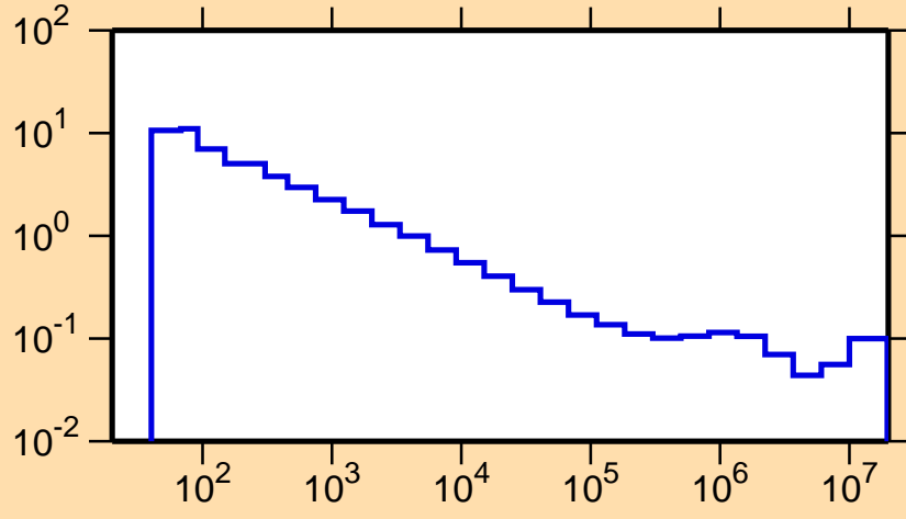
\sigma vs. E for ^{135}\text{Sm}(n,\alpha)
