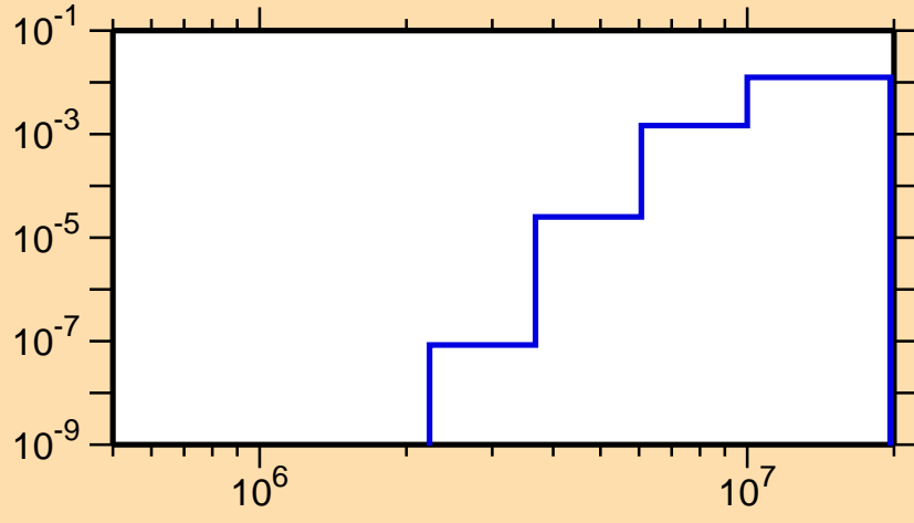
\sigma vs. E for ^{135}\text{Sm}(n,n\alpha)
