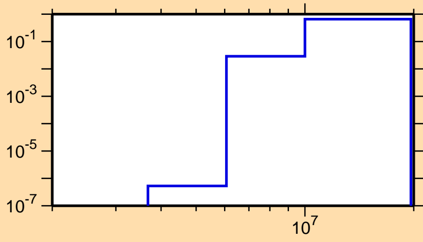
\sigma vs. E for ^{135}\text{Sm}(n,np)
