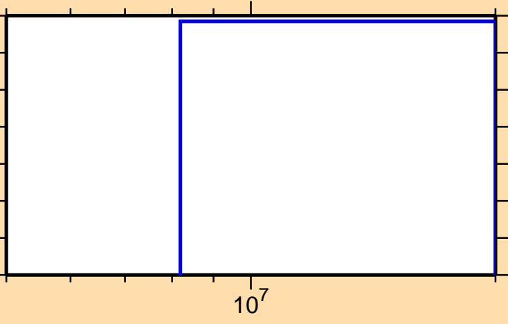
\sigma vs. E for ^{135}\text{Sm}(n,\text{nd})
