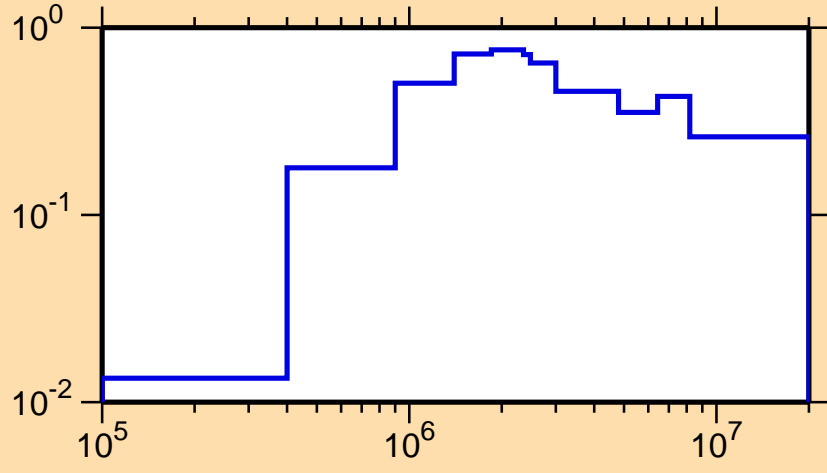
\sigma vs. E for ^{135}\text{Sm}(n,n\text{cont.})
