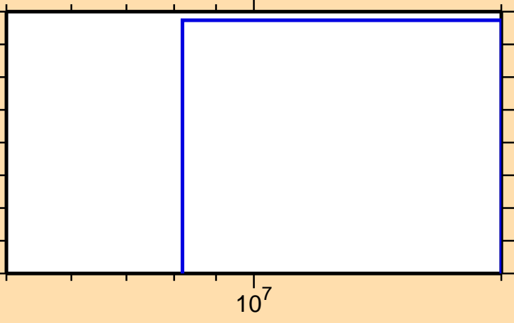
\sigma vs. E for ^{135}\text{Sm}(n,2n\alpha)
