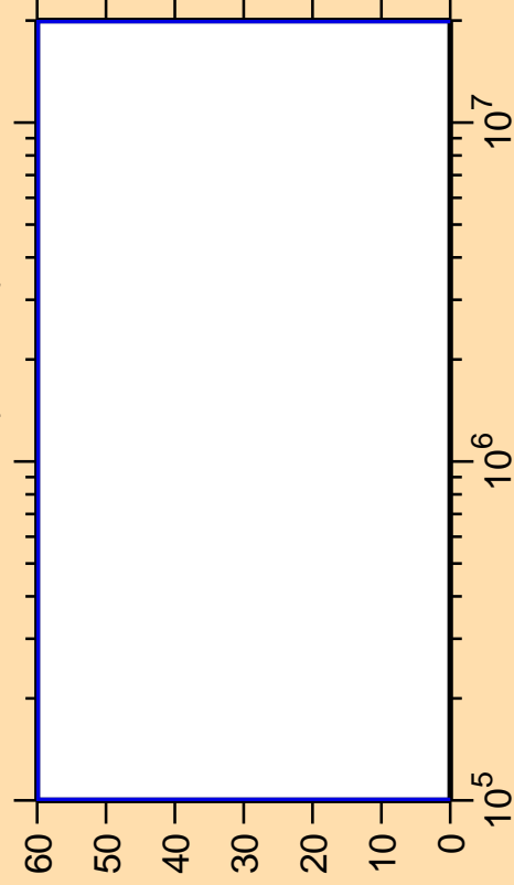
\Delta\sigma/\sigma vs. E for ^{135}\text{Sm}(n,\text{inel.})
