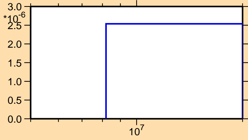
\sigma vs. E for ^{135}\text{Sm}(n,\text{pt})
