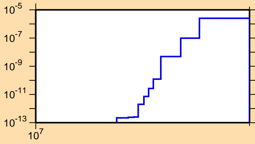
\sigma vs. E for ^{136}\text{Sm}(n,2n\alpha)
