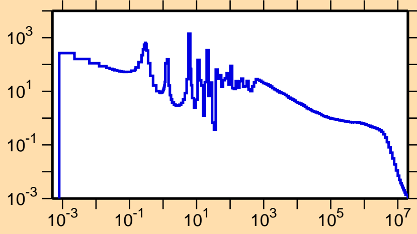
\sigma vs. E for ^{136}\text{Sm}(n,\gamma)
