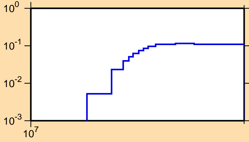
\sigma vs. E for ^{136}\text{Sm}(n,2n)
