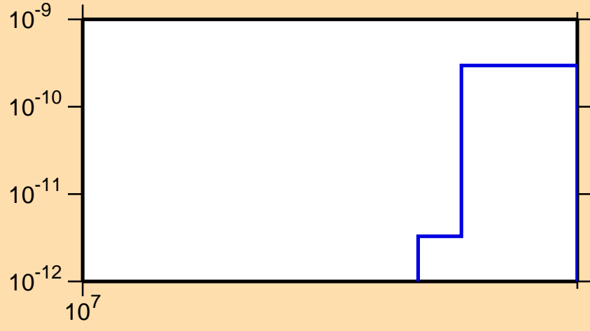
\sigma vs. E for ^{136}\text{Sm} (mt 34)
