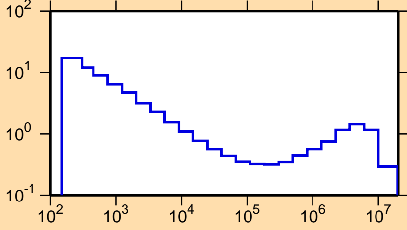
\sigma vs. E for ^{136}\text{Sm}(n,p)
