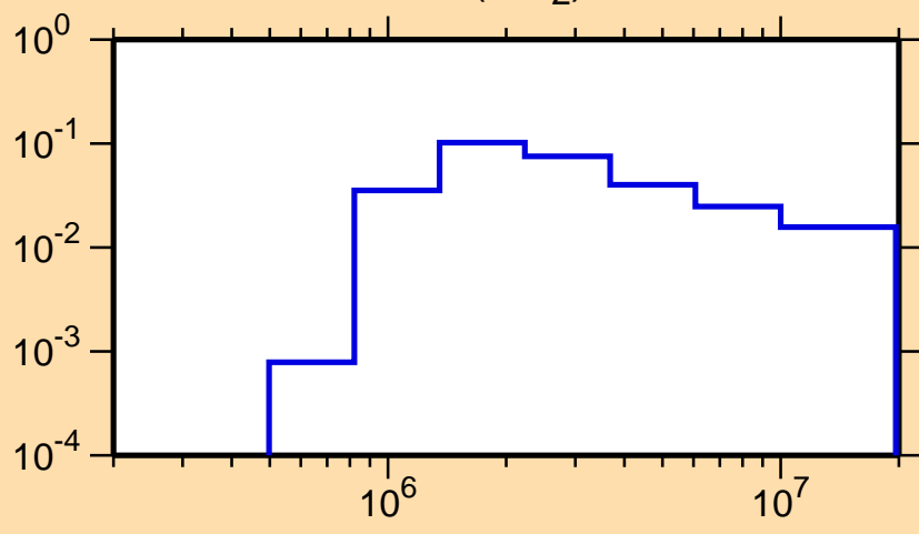
\sigma vs. E for ^{136}\text{Sm}(n,n_2)
