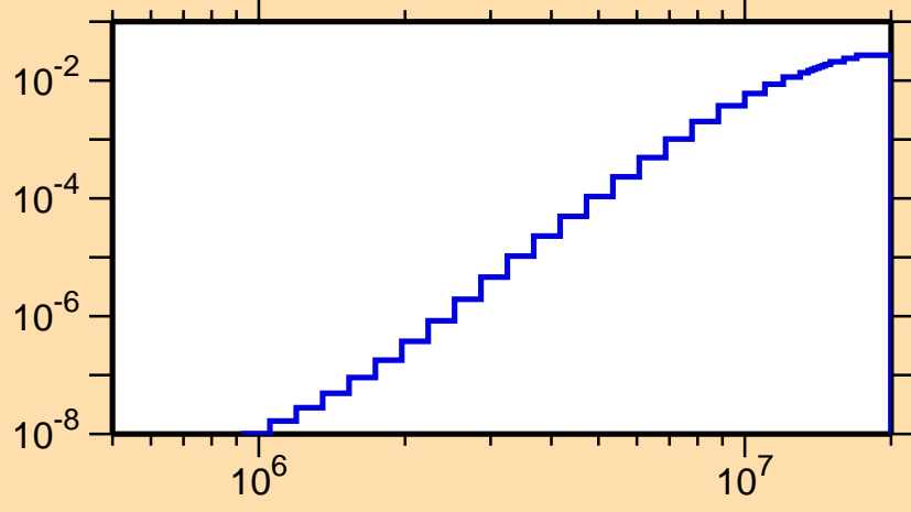
\sigma vs. E for ^{137}\text{Sm}(n,p\alpha)
