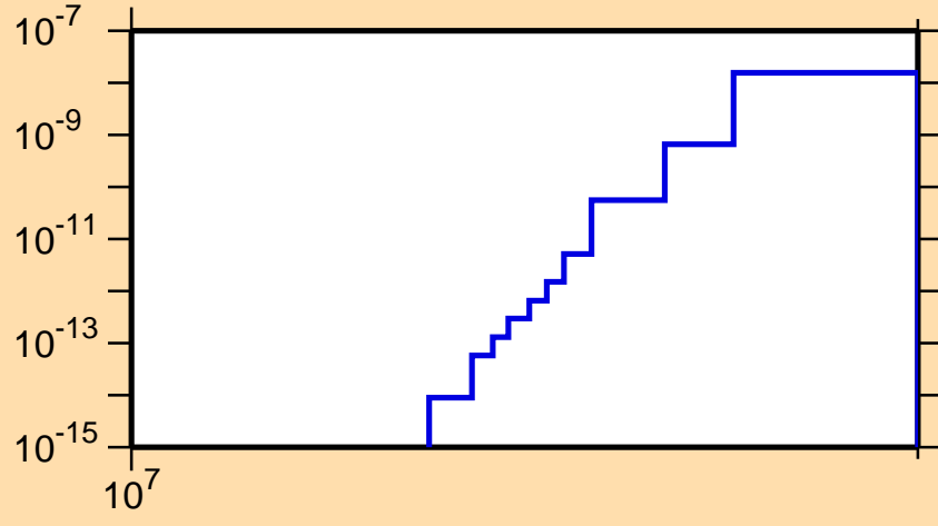
\sigma vs. E for ^{137}\text{Sm} (mt 34)
