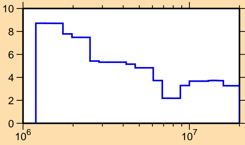
\Delta\sigma/\sigma vs. E for ^{137}\text{Sm}(n, \text{tot.})
