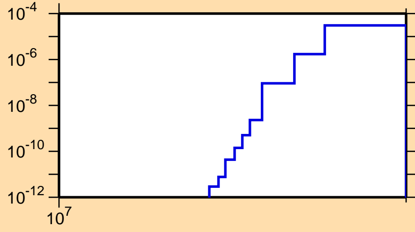
\sigma vs. E for ^{137}\text{Sm}(n,\text{pt})
