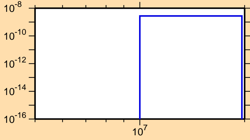
\sigma vs. E for ^{137}\text{Sm}(\text{mt117})
