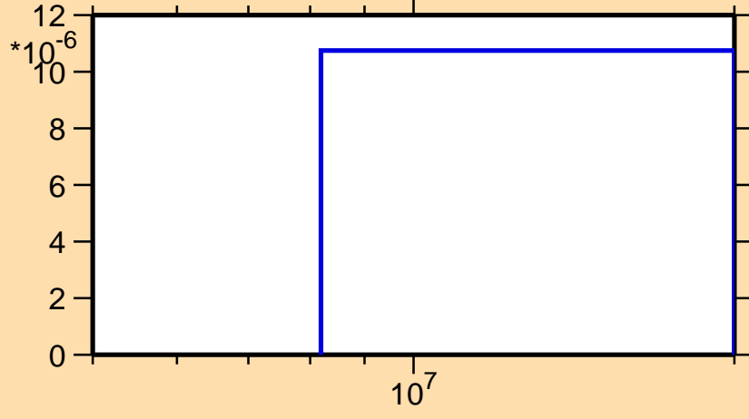
\sigma vs. E for ^{137}\text{Sm}(n,\text{pd})
