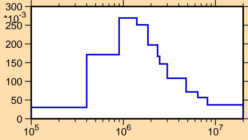
\sigma vs. E for ^{137}\text{Sm}(n,n_1)
