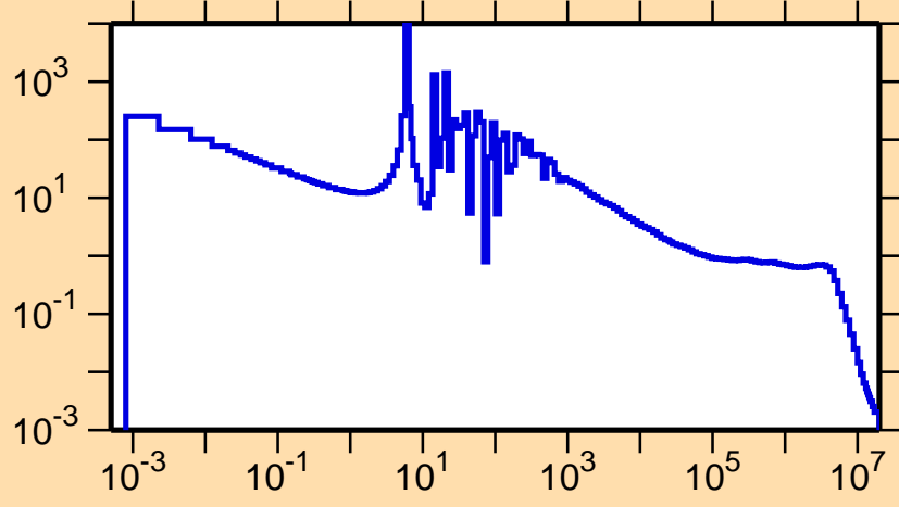
\sigma vs. E for ^{138}\text{Sm}(n,\gamma)
