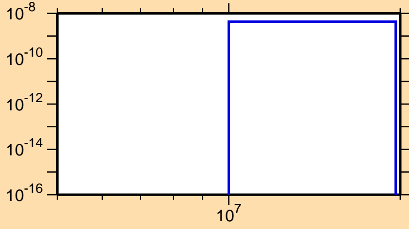
\sigma vs. E for ^{138}\text{Sm}(\text{mt117})
