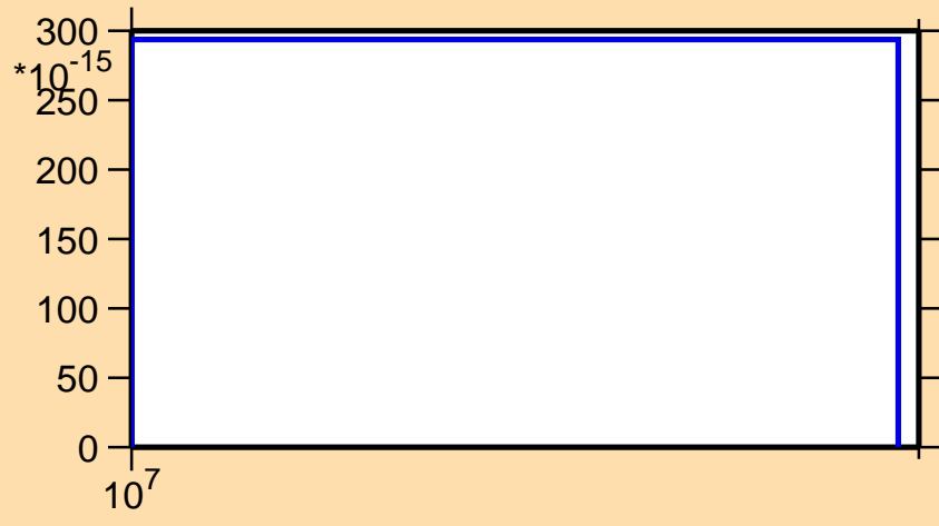
\sigma vs. E for ^{138}\text{Sm} (mt 34)
