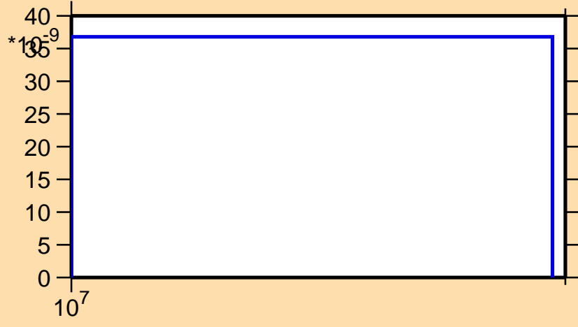
\sigma vs. E for ^{138}\text{Sm}(n,2n\alpha)
