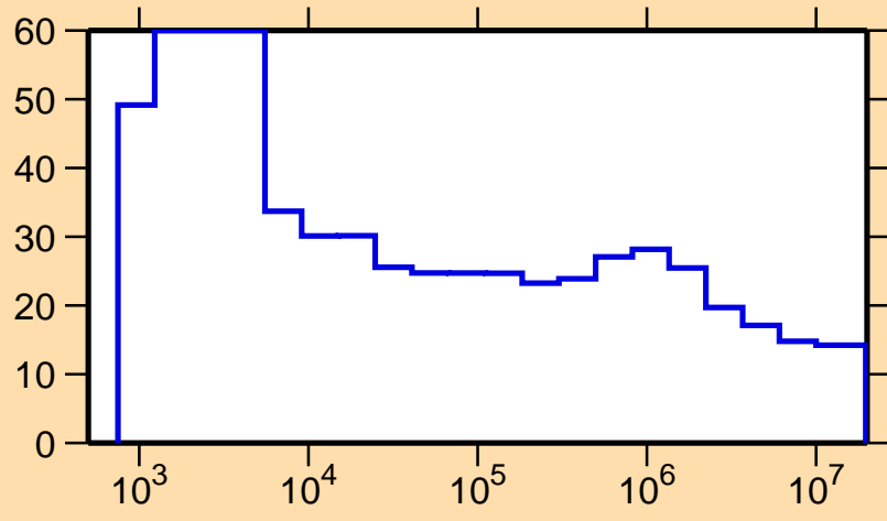
\Delta\sigma/\sigma vs. E for ^{138}\text{Sm}(n,\text{nonel.})
