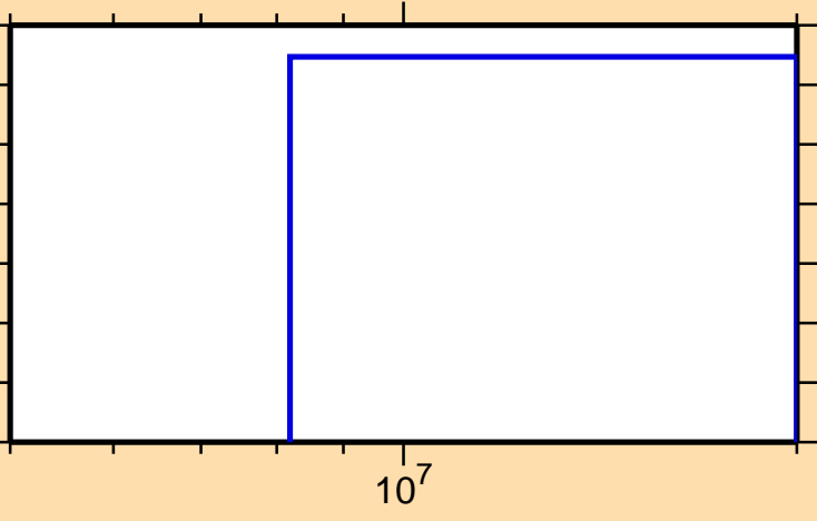
\sigma vs. E for ^{138}\text{Sm} (mt 45)
