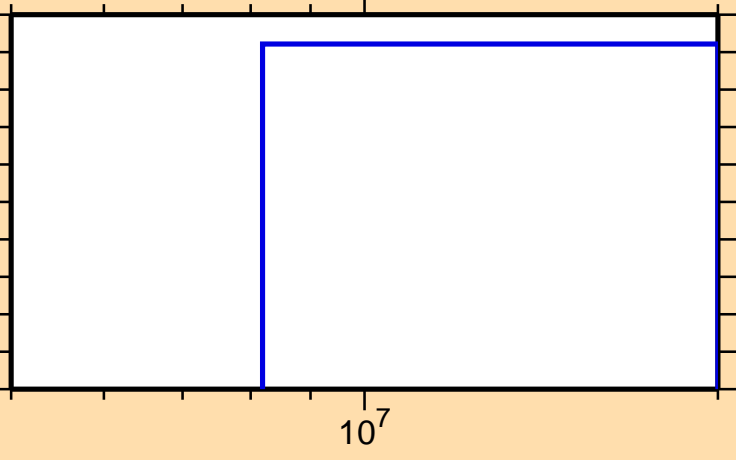
\sigma vs. E for ^{138}\text{Sm}(n,t)
