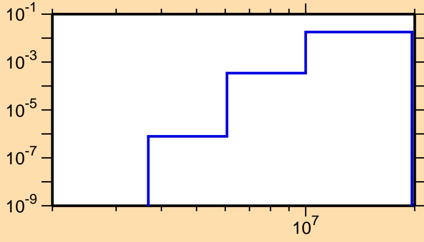
\sigma vs. E for ^{139}\text{Sm}(n,n\alpha)
