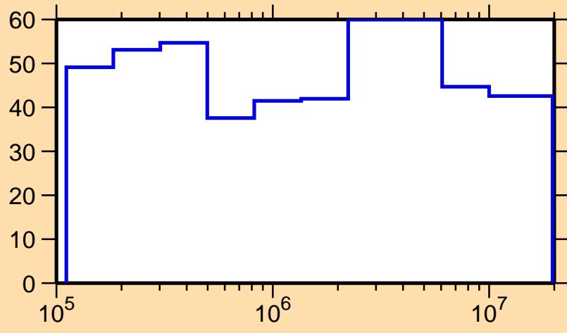
\Delta\sigma/\sigma vs. E for ^{139}\text{Sm}(n,n_1)
