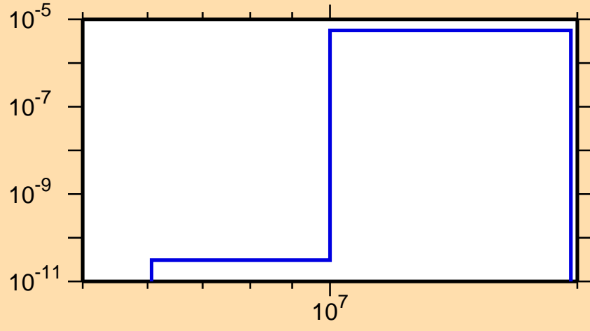
\sigma vs. E for ^{139}\text{Sm}(n,\text{He}3)
