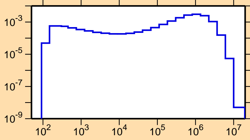
\sigma vs. E for ^{139}\text{Sm}(n,n_3)
