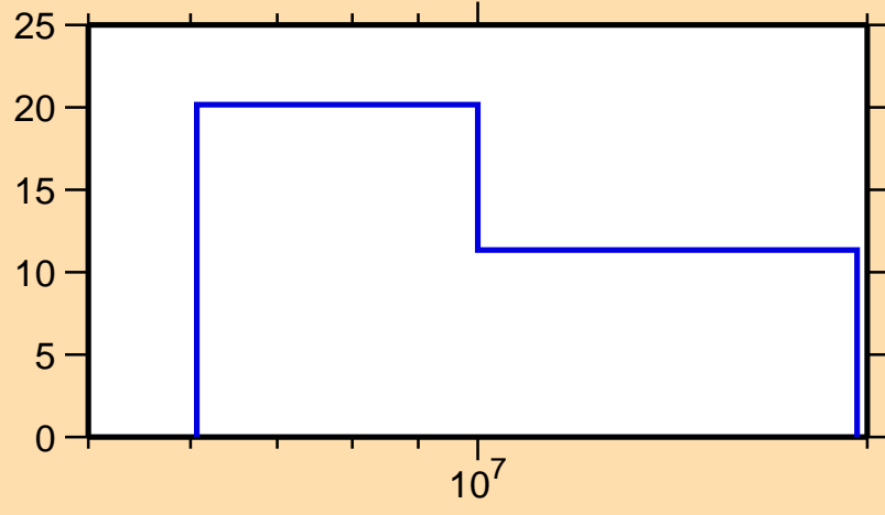
\Delta\sigma/\sigma vs. E for ^{139}\text{Sm}(n,\text{el.})
