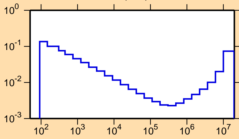
\sigma vs. E for ^{139}\text{Sm}(n,\alpha)
