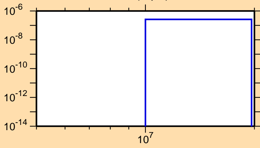
\sigma vs. E for ^{139}\text{Sm}(n,pd)
