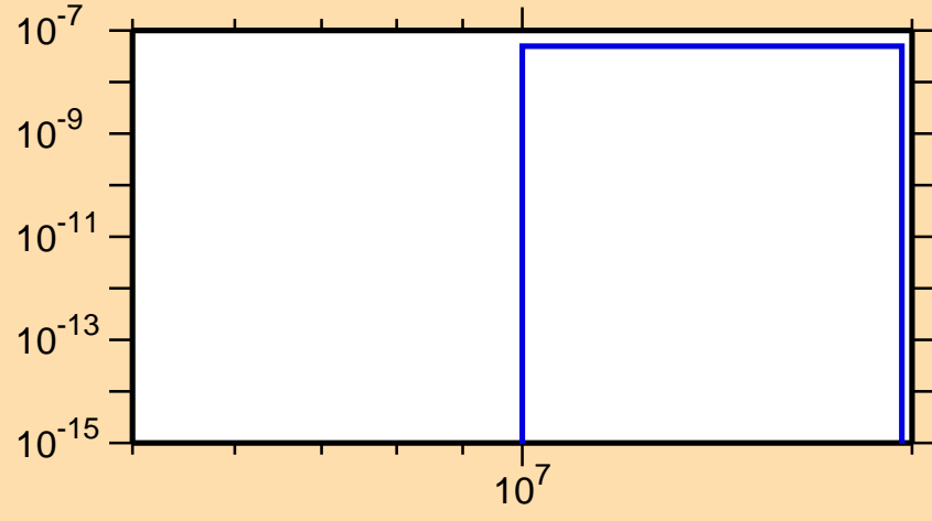
\sigma vs. E for ^{139}\text{Sm} (mt 45)
