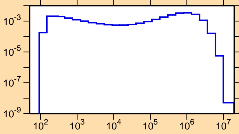
\sigma vs. E for ^{139}\text{Sm}(n,n_2)
