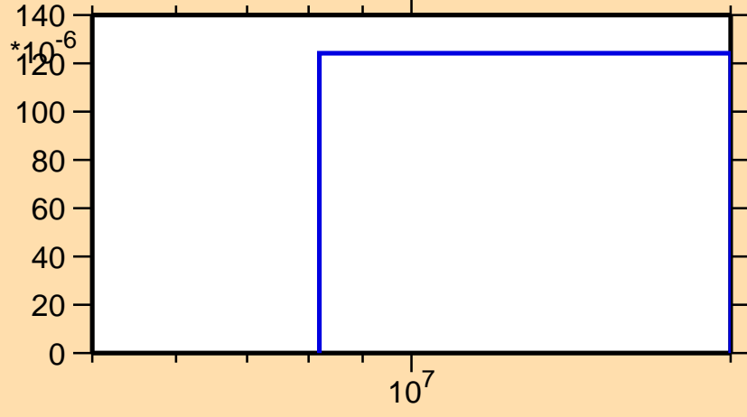
\sigma vs. E for ^{139}\text{Sm}(n,t)
