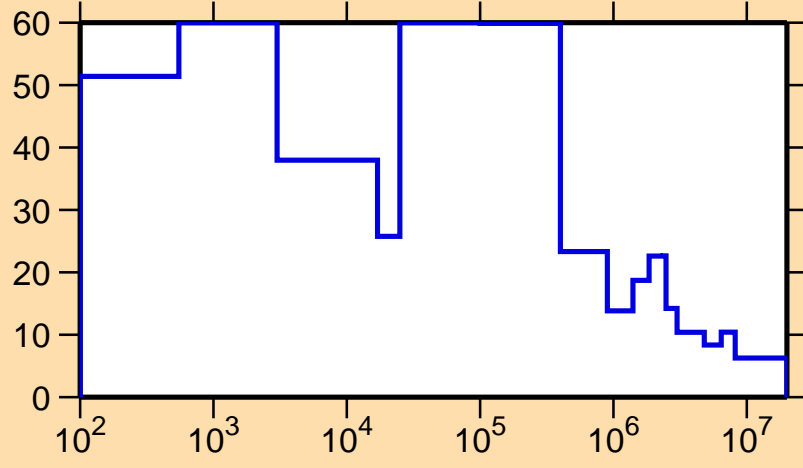
\Delta\sigma/\sigma vs. E for ^{139}\text{Sm}(n,\text{tot.})
