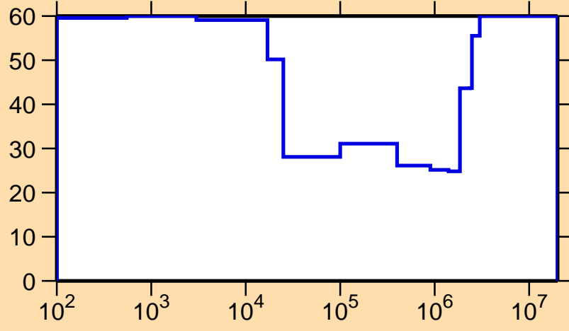
\Delta\sigma/\sigma vs. E for ^{139}\text{Sm}(n,\gamma)
