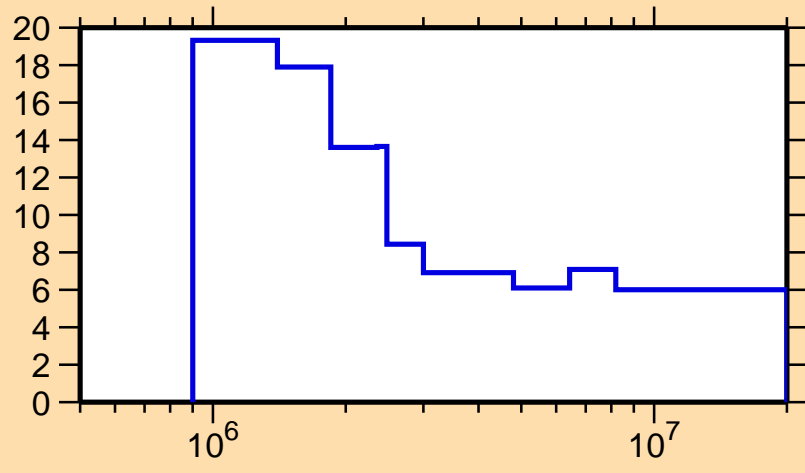
\Delta\sigma/\sigma vs. E for ^{139}\text{Sm}(n,\text{nonel.})
