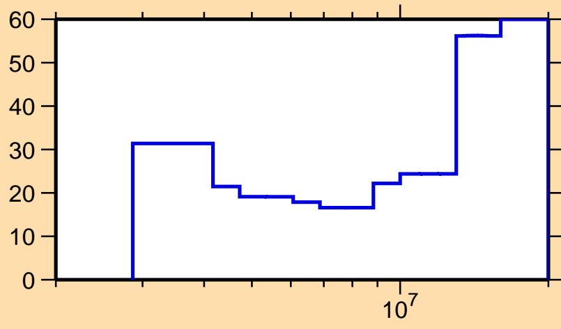
\Delta\sigma/\sigma vs. E for ^{140}\text{Sm}(n,n\text{cont.})
