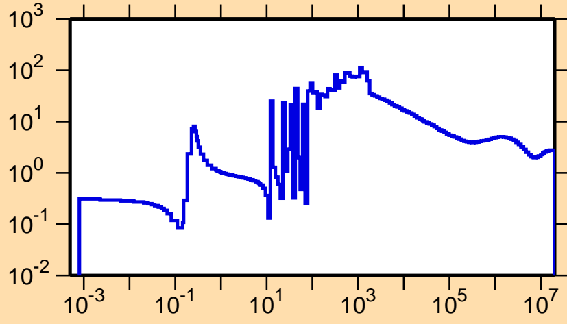
\sigma vs. E for ^{140}\text{Sm}(n,\text{el.})
