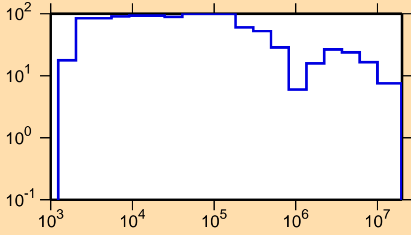
\Delta\sigma/\sigma vs. E for ^{140}\text{Sm}(n,el.)
