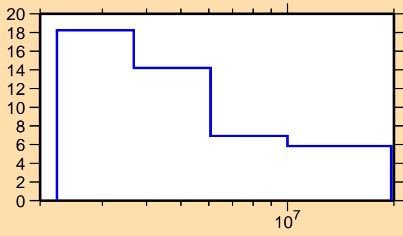
\Delta\sigma/\sigma vs. E for ^{140}\text{Sm}(n,\text{tot.})
