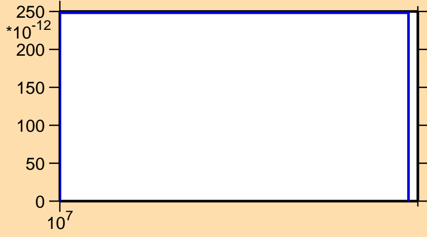
\sigma vs. E for ^{140}\text{Sm}(\text{mt117})
