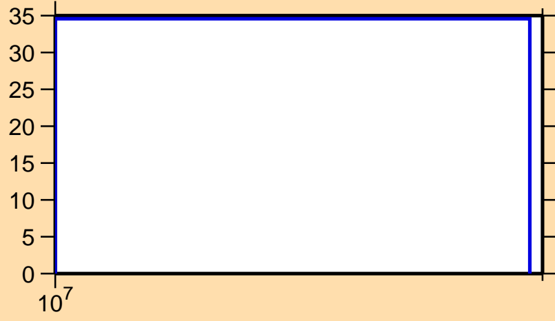
\Delta\sigma/\sigma vs. E for ^{140}\text{Sm}(n,\text{inel.})
