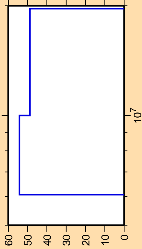
\Delta\sigma/\sigma vs. E for ^{140}\text{Sm}(n,np)
