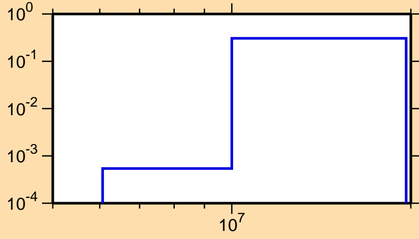
\sigma vs. E for ^{140}\text{Sm}(n,np)
