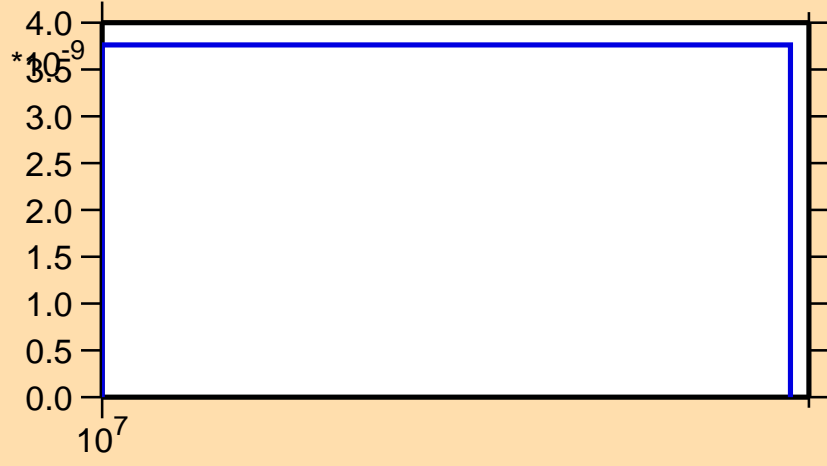
\sigma vs. E for ^{140}\text{Sm}(n,2np)
