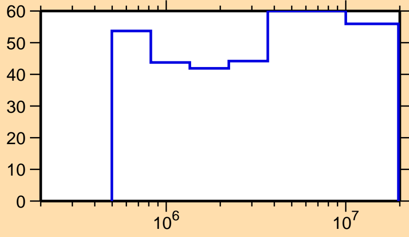
\Delta\sigma/\sigma vs. E for ^{140}\text{Sm}(n,n_1)
