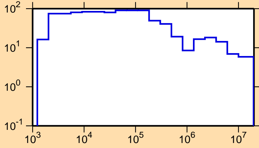
\Delta\sigma/\sigma vs. E for ^{140}\text{Sm}(n,\text{tot.})
