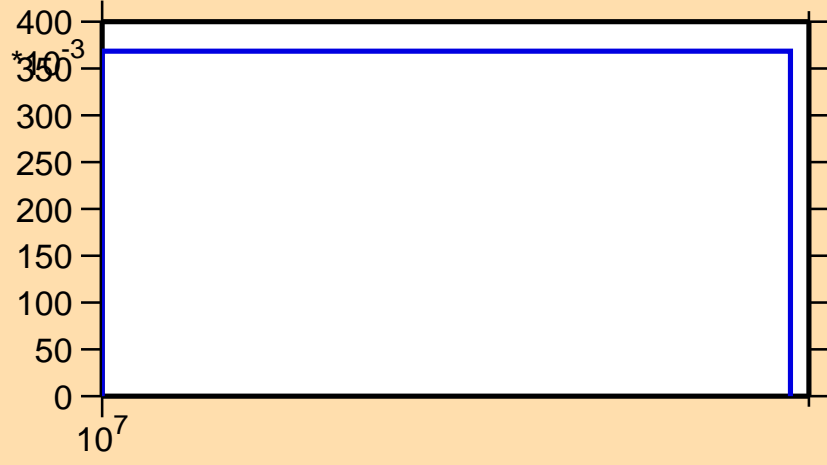
\sigma vs. E for ^{140}\text{Sm}(n,2n)
