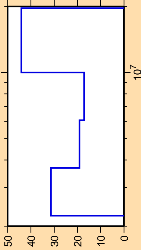
\Delta\sigma/\sigma vs. E for ^{140}\text{Sm}(n,n\text{cont.})
