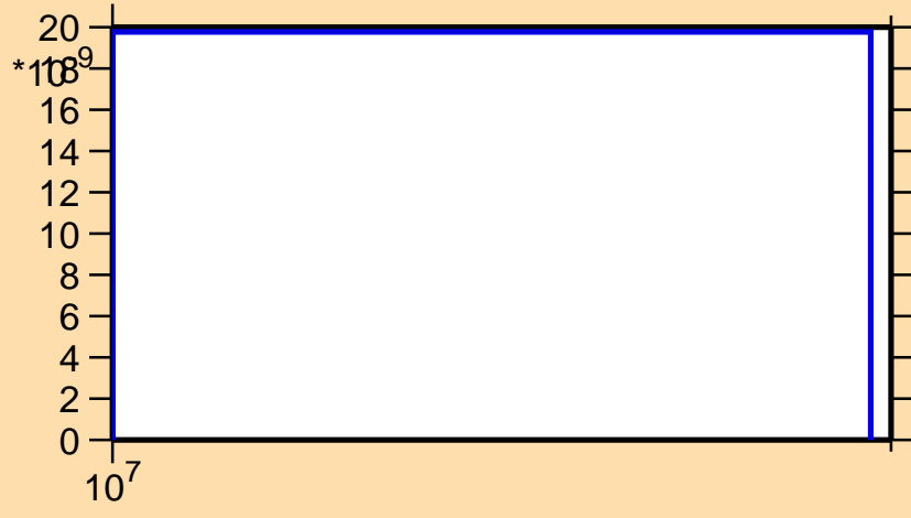
\sigma vs. E for ^{140}\text{Sm}(n,2n\alpha)
