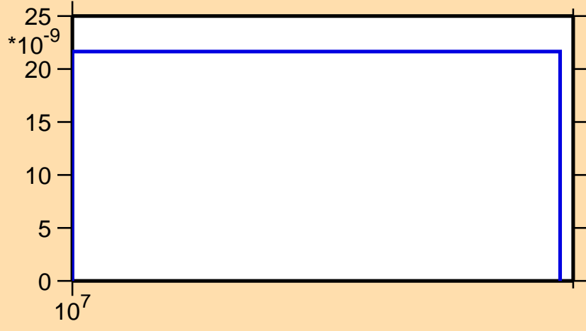
\sigma vs. E for ^{140}\text{Sm} (mt 45)
