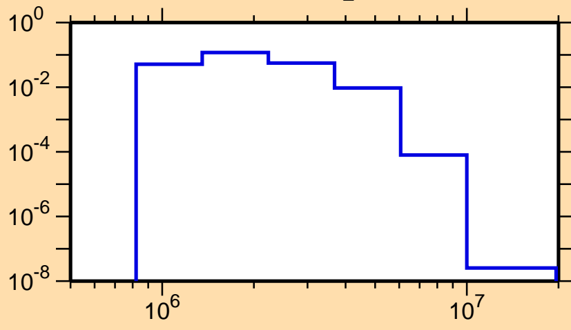
\sigma vs. E for ^{140}\text{Sm}(n,n_2)
