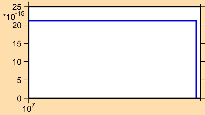
\sigma vs. E for ^{140}\text{Sm} (mt 34)
