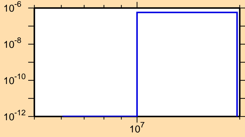
\sigma vs. E for ^{140}\text{Sm}(n,\text{He}3)
