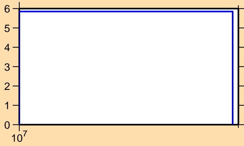
\Delta\sigma/\sigma vs. E for ^{140}\text{Sm}(n,\text{tot.})
