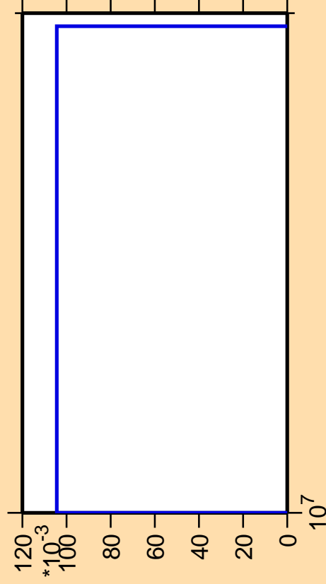
\Delta\sigma/\sigma vs. E for ^{140}\text{Sm} (mt 34)
