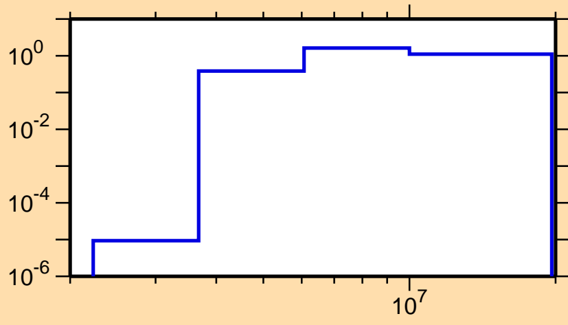
\sigma vs. E for ^{140}\text{Sm}(n,n\text{cont.})
