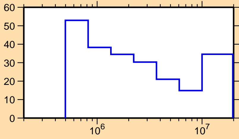
\Delta\sigma/\sigma vs. E for ^{140}\text{Sm}(n,\text{inel.})
