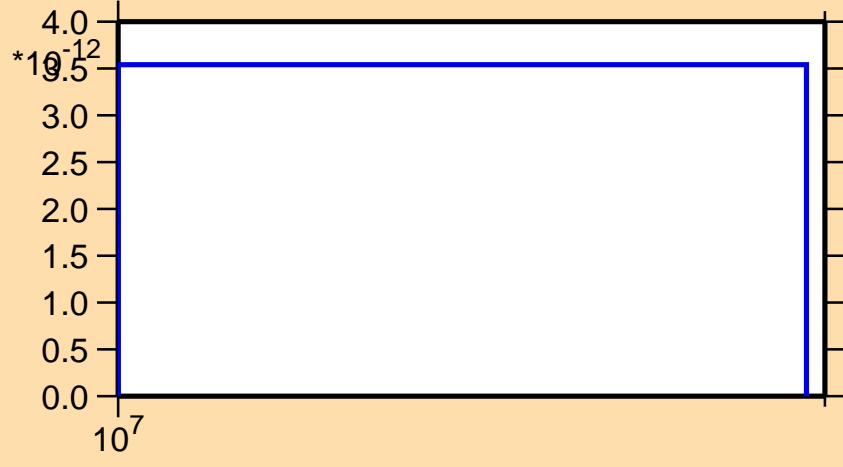
\sigma vs. E for ^{140}\text{Sm}(n,\text{pt})
