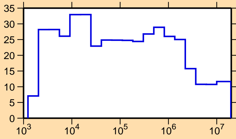
\Delta\sigma/\sigma vs. E for ^{140}\text{Sm}(n,\text{nonel.})
