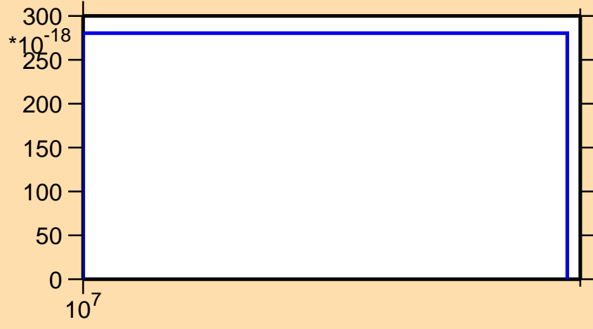
\sigma vs. E for ^{140}\text{Sm}(n,nt)
