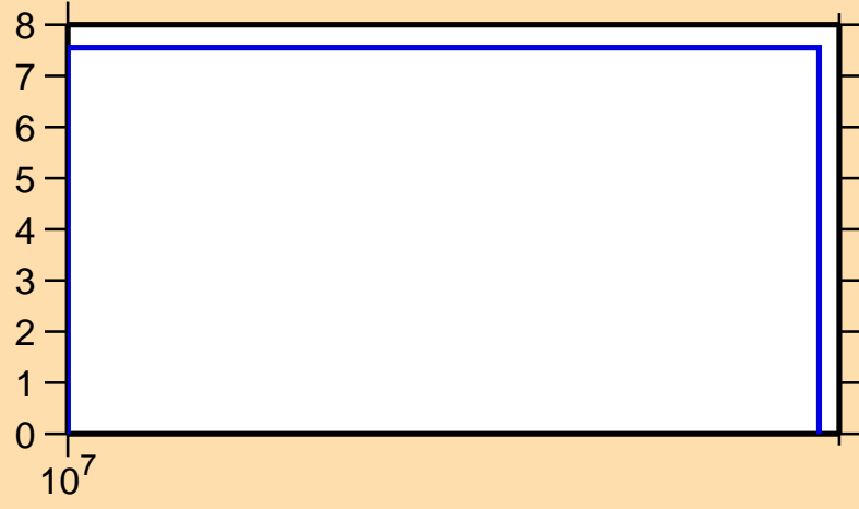
\Delta\sigma/\sigma vs. E for ^{140}\text{Sm}(n,\text{el.})
