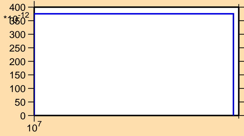
\sigma vs. E for ^{140}\text{Sm}(n,\text{nd})
