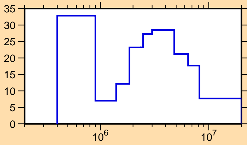
\Delta\sigma/\sigma vs. E for ^{140}\text{Sm}(n,\text{el.})
