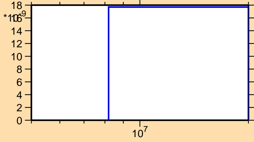
\sigma vs. E for ^{140}\text{Sm}(n,2n\alpha)
