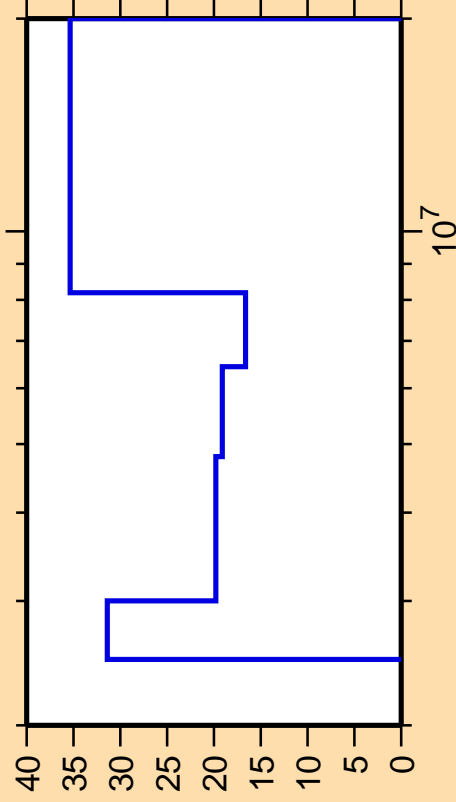
\Delta\sigma/\sigma vs. E for ^{140}\text{Sm}(n,n\text{cont.})
