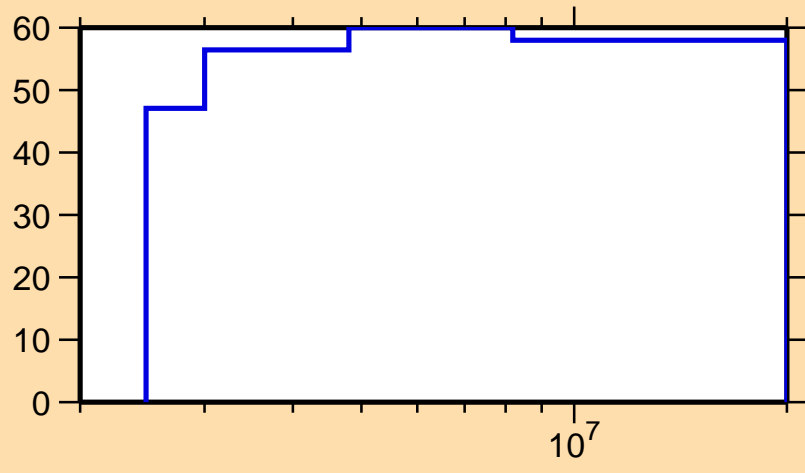
\Delta\sigma/\sigma vs. E for ^{140}\text{Sm}(n,n_1)
