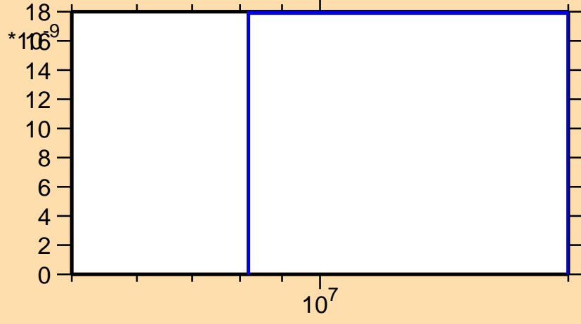
\sigma vs. E for ^{140}\text{Sm} (mt 45)
