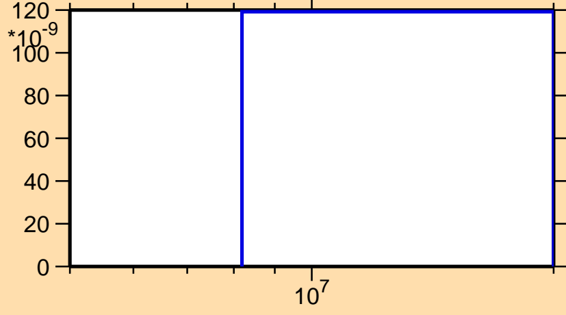
\sigma vs. E for ^{140}\text{Sm}(n,\text{pd})
