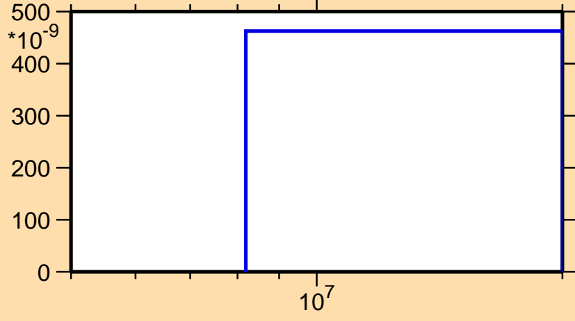
\sigma vs. E for ^{140}\text{Sm}(n,\text{He}3)
