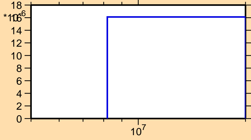
\sigma vs. E for ^{140}\text{Sm}(n,t)
