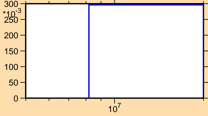
\sigma vs. E for ^{140}\text{Sm}(n,2n)
