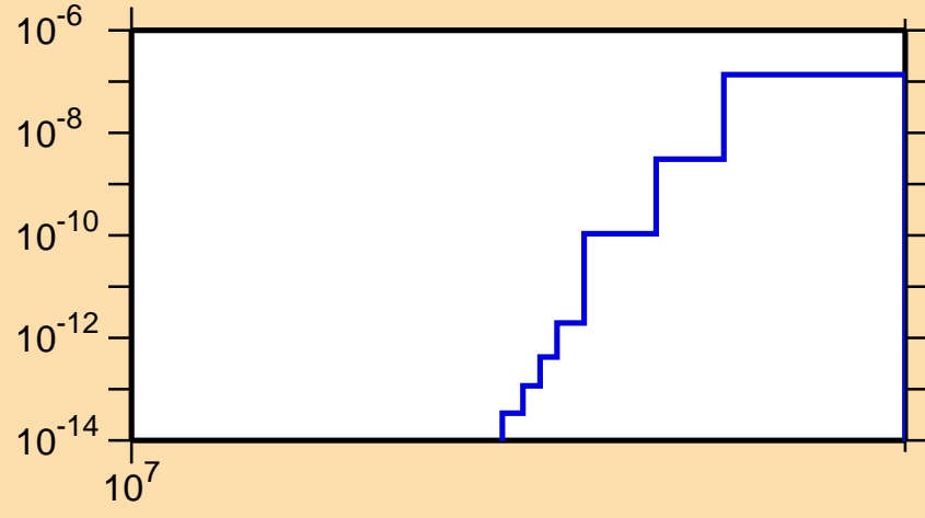
\sigma vs. E for ^{141}\text{Sm}(n,pt)
