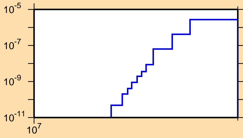
\sigma vs. E for ^{141}\text{Sm}(n,\text{pd})
