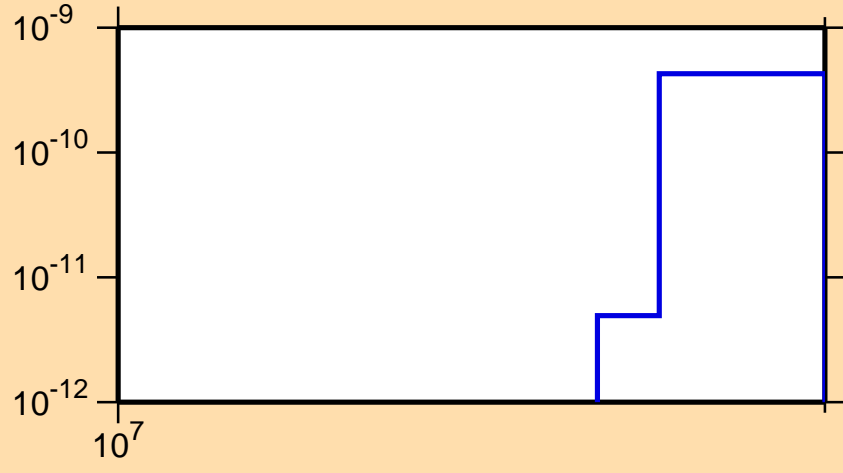
\sigma vs. E for ^{141}\text{Sm} (mt 34)
