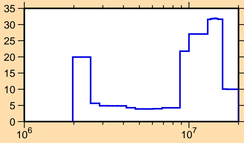
\Delta\sigma/\sigma vs. E for ^{141}\text{Sm}(n,n\text{cont.})
