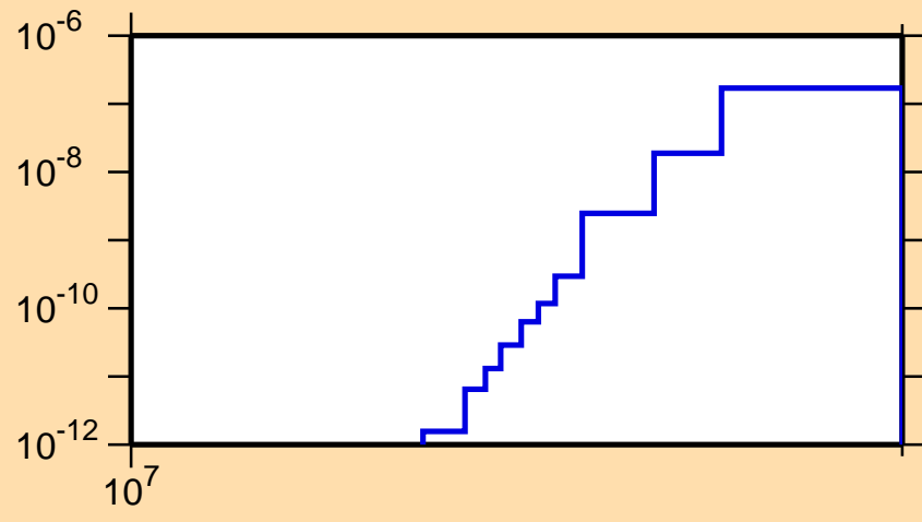
\sigma vs. E for ^{141}\text{Sm} (mt 45)
