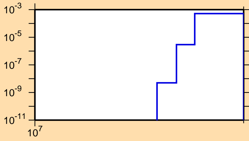
\sigma vs. E for ^{141}\text{Sm}(n,2np)
