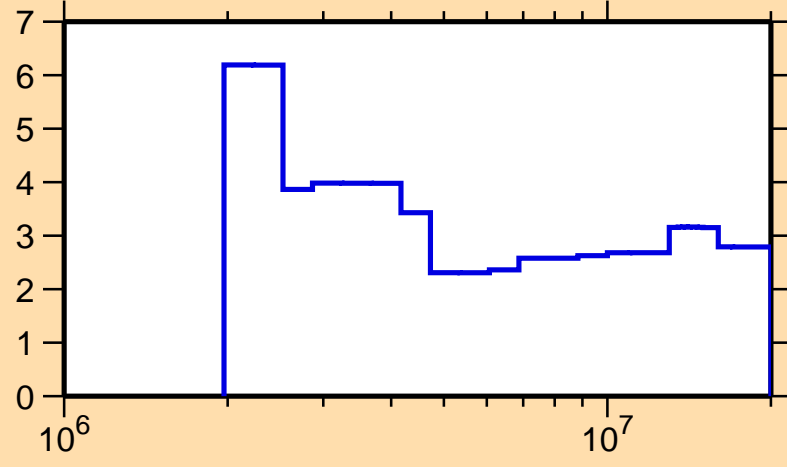
\Delta\sigma/\sigma vs. E for ^{141}\text{Sm}(n,\text{nonel.})
