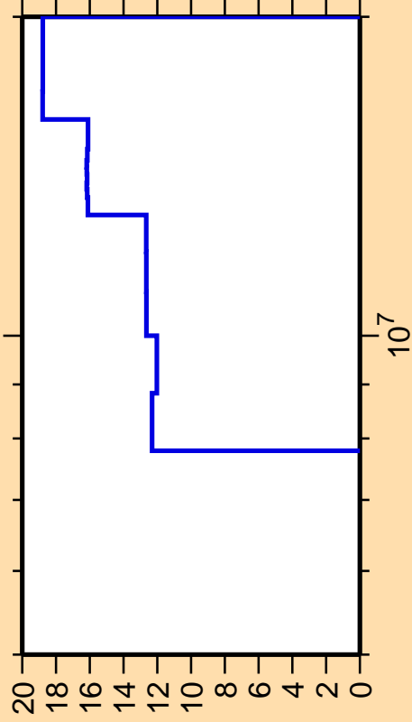
\Delta\sigma/\sigma vs. E for ^{141}\text{Sm}(n,p)
