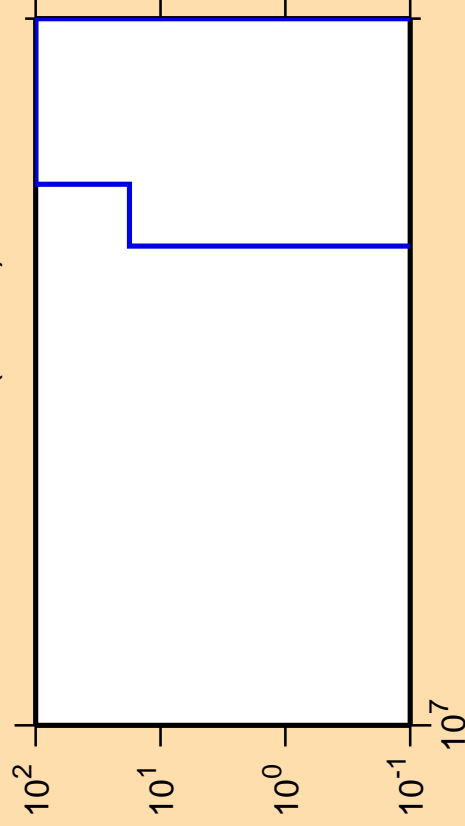
\Delta\sigma/\sigma vs. E for ^{141}\text{Sm} (mt 34)
