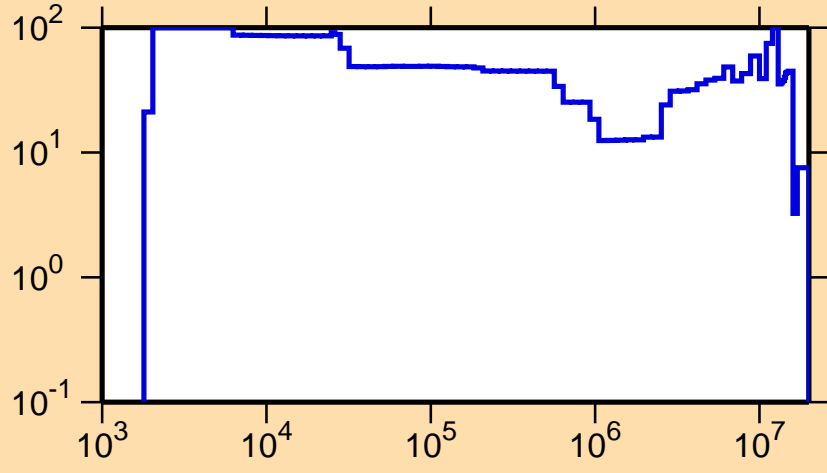
\Delta\sigma/\sigma vs. E for ^{141}\text{Sm}(n,n_1)
