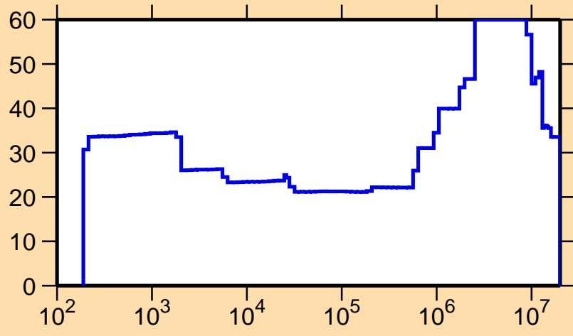
\Delta\sigma/\sigma vs. E for ^{141}\text{Sm}(n,\gamma)
