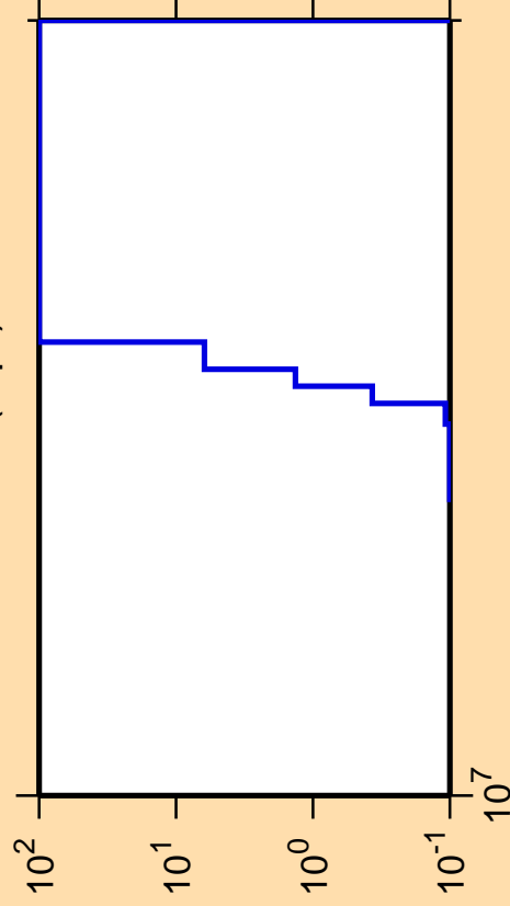
\Delta\sigma/\sigma vs. E for ^{141}\text{Sm}(n,pt)
