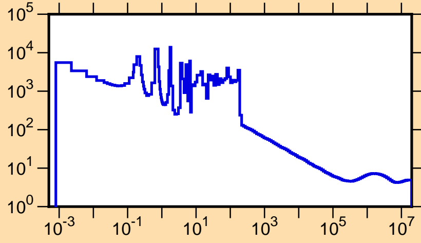
\sigma vs. E for ^{141}\text{Sm}(n,\text{tot.})
