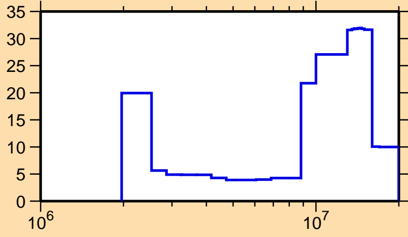
\Delta\sigma/\sigma vs. E for ^{141}\text{Sm}(n,n\text{cont.})
