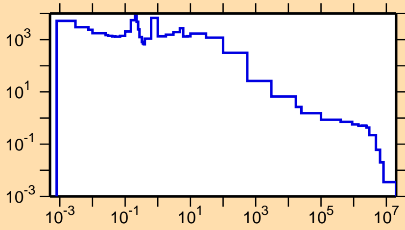
\sigma vs. E for ^{141}\text{Sm}(n,\gamma)
