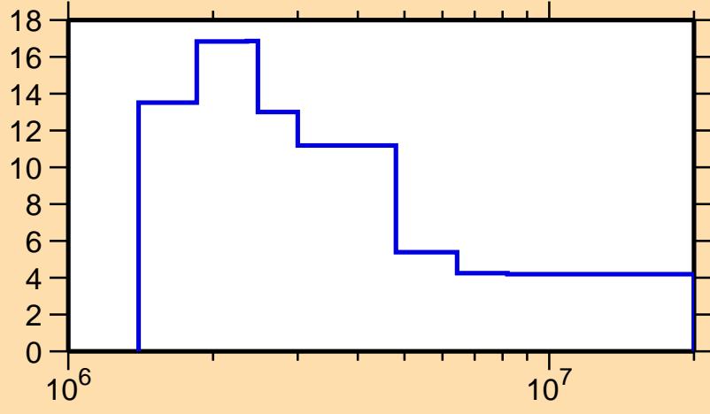
\Delta\sigma/\sigma vs. E for ^{141}\text{Sm}(n,\text{tot.})
