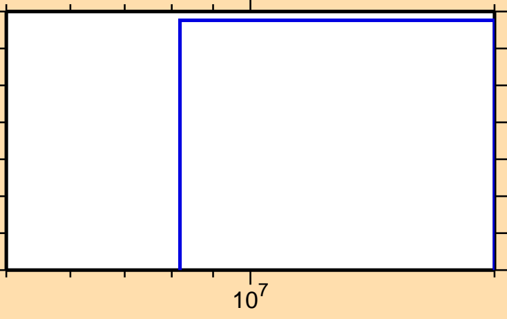
\sigma vs. E for ^{141}\text{Sm}(n,\text{nd})
