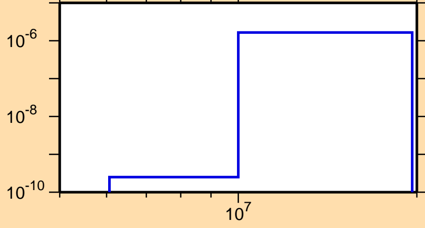
\sigma vs. E for ^{142}\text{Sm}(n,p\alpha)
