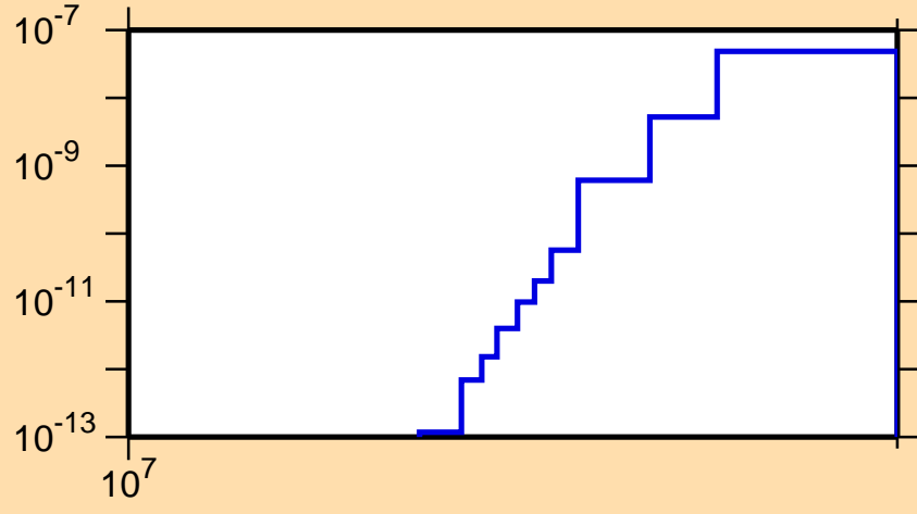
\sigma vs. E for ^{143}\text{Sm}(n,\text{pd})
