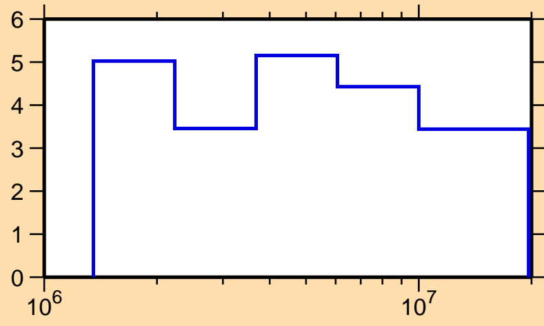
\Delta\sigma/\sigma vs. E for ^{143}\text{Sm}(n,n\text{onel.})
