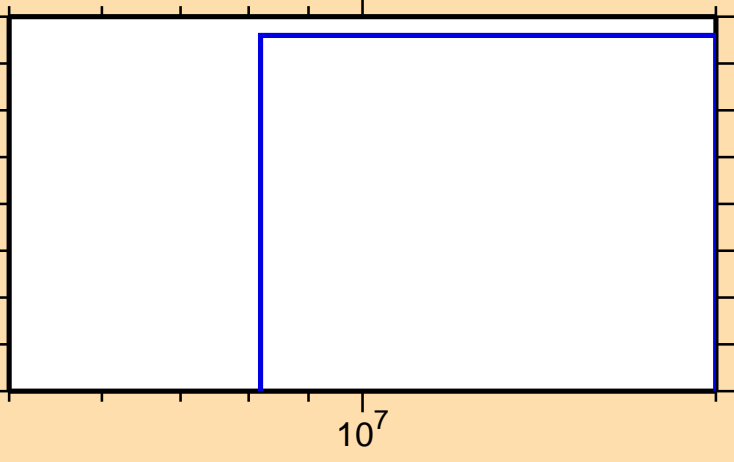
\sigma vs. E for ^{143}\text{Sm}(n,nt)
