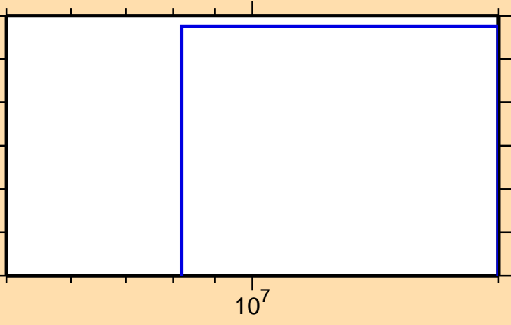
\sigma vs. E for ^{143}\text{Sm}(n,\text{He3})
