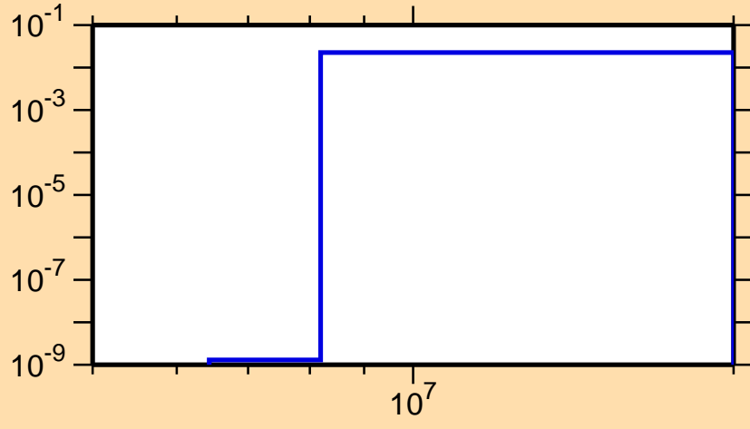
\sigma vs. E for ^{144}\text{Sm}(n,np)
