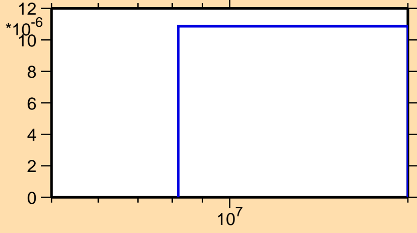
\sigma vs. E for ^{144}\text{Sm}(n,t)
