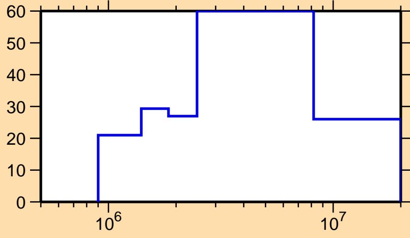
\Delta\sigma/\sigma vs. E for ^{144}\text{Sm}(n,p)
