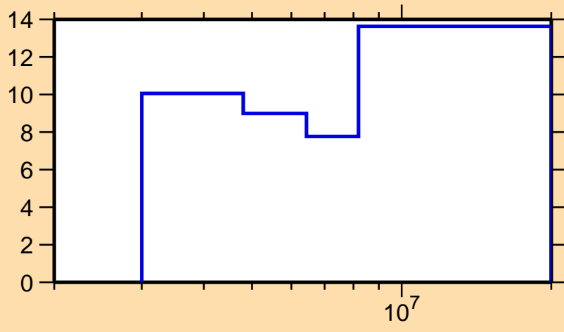
\Delta\sigma/\sigma vs. E for ^{144}\text{Sm}(n,n\text{cont.})
