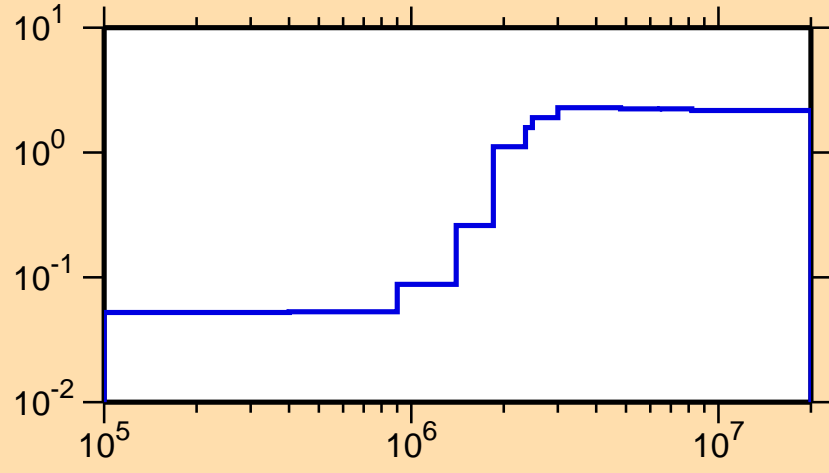
\sigma vs. E for ^{144}\text{Sm}(n,\text{nonel.})
