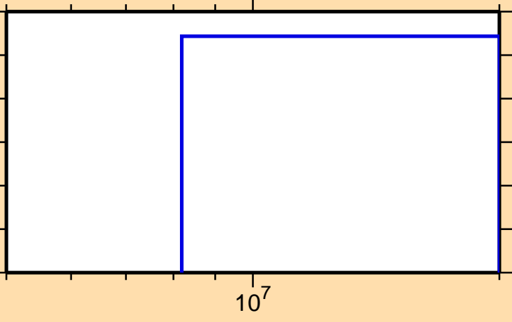
\sigma vs. E for ^{144}\text{Sm}(n,t)
