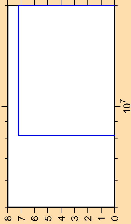
\Delta\sigma/\sigma vs. E for ^{144}\text{Sm}(n,2n)
