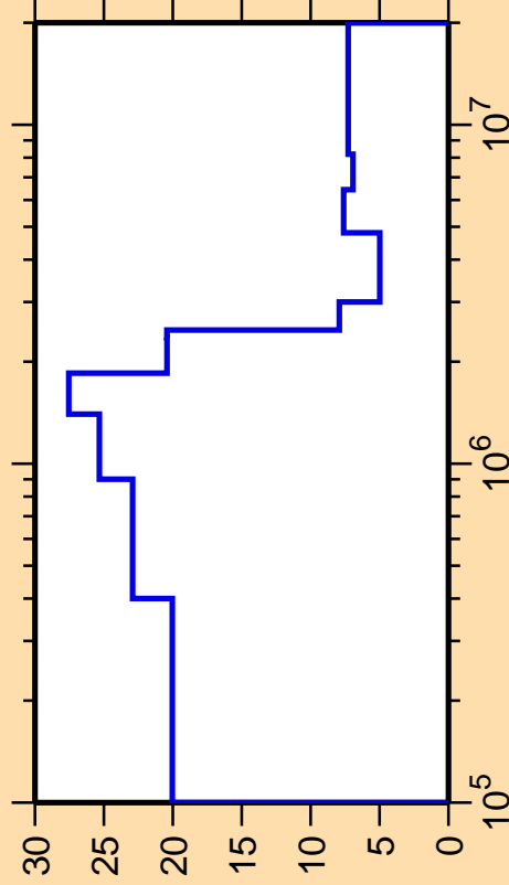
\Delta\sigma/\sigma vs. E for ^{144}\text{Sm}(n,\text{nonel.})
