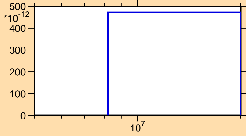
\sigma vs. E for ^{144}\text{Sm}(n,2np)
