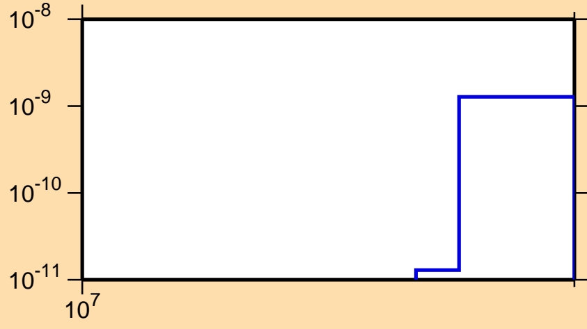
\sigma vs. E for ^{145}\text{Sm}(n,\text{pt})
