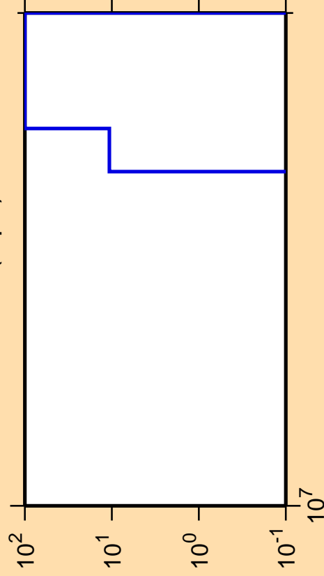
\Delta\sigma/\sigma vs. E for ^{145}\text{Sm}(n,\text{pd})
