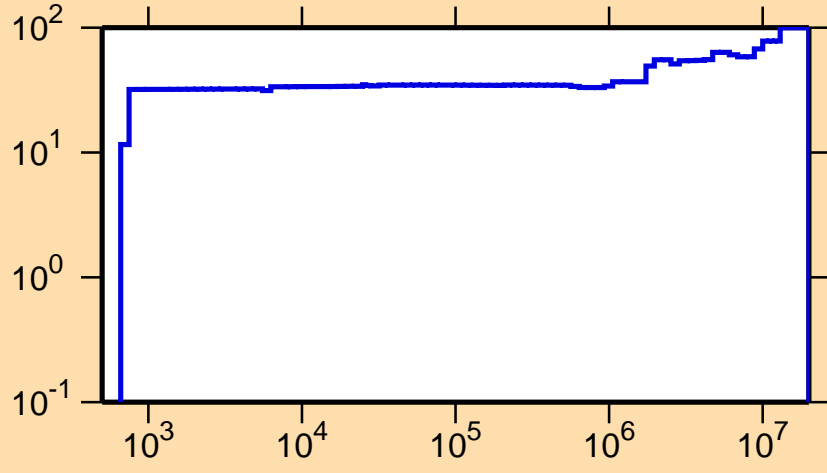
\Delta\sigma/\sigma vs. E for ^{145}\text{Sm}(n,\gamma)
