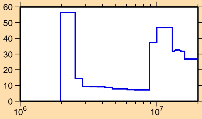
\Delta\sigma/\sigma vs. E for ^{145}\text{Sm}(n,n\text{cont.})
