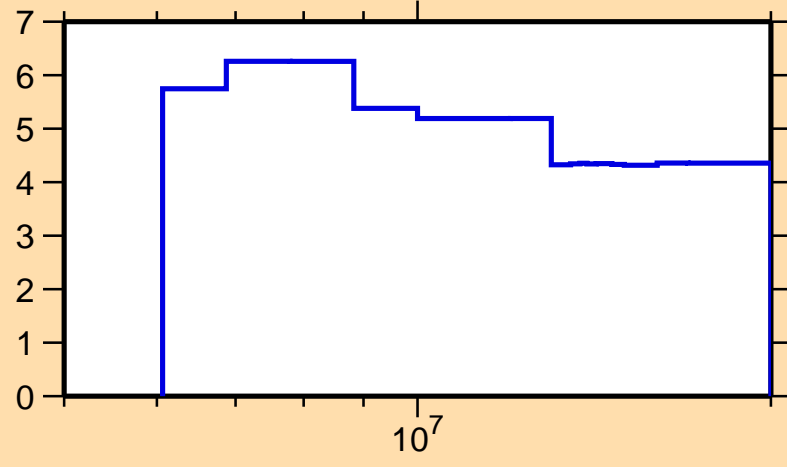
\Delta\sigma/\sigma vs. E for ^{145}\text{Sm}(n,\text{nonel.})
