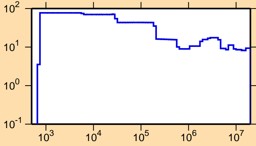
\Delta\sigma/\sigma vs. E for ^{145}\text{Sm}(n,el.)
