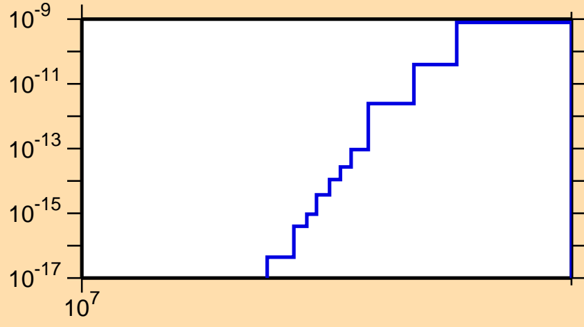
\sigma vs. E for ^{145}\text{Sm} (mt 45)
