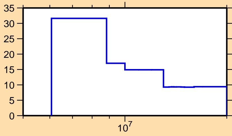
\Delta\sigma/\sigma vs. E for ^{145}\text{Sm}(n,2n)
