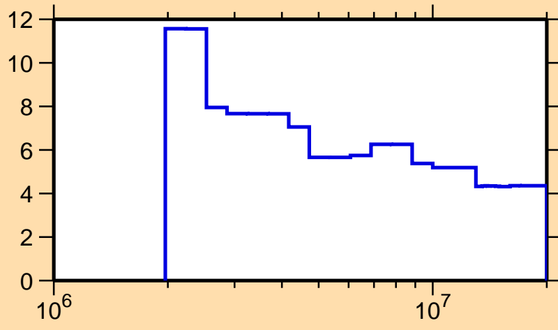
\Delta\sigma/\sigma vs. E for ^{145}\text{Sm}(n,\text{nonel.})
