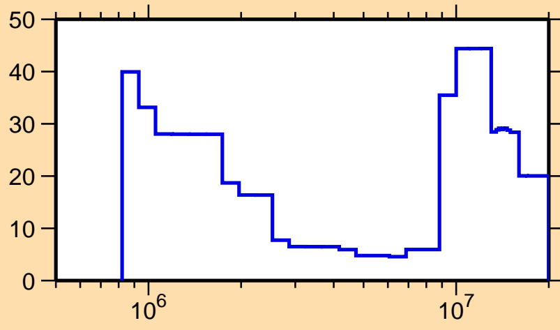
\Delta\sigma/\sigma vs. E for ^{145}\text{Sm}(n,\text{inel.})
