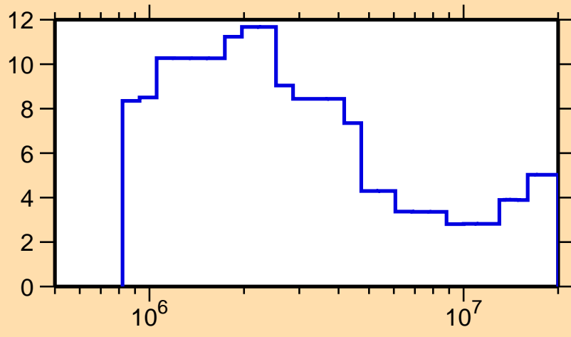
\Delta\sigma/\sigma vs. E for ^{145}\text{Sm}(n,\text{tot.})
