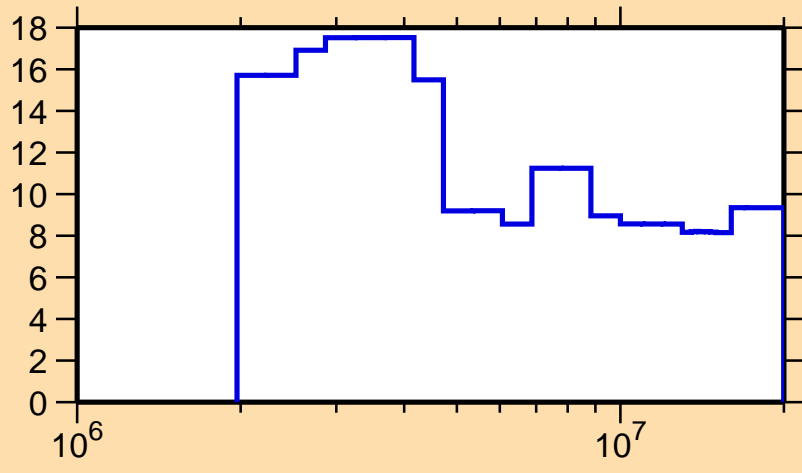
\Delta\sigma/\sigma vs. E for ^{145}\text{Sm}(n,\text{el.})
