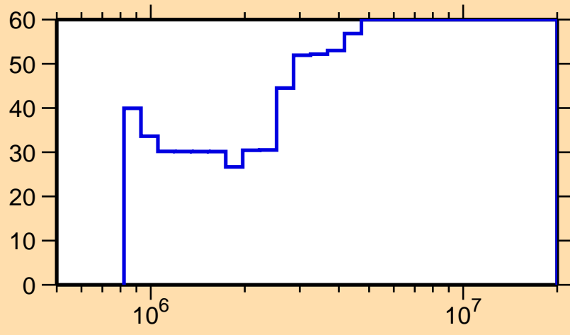
\Delta\sigma/\sigma vs. E for ^{145}\text{Sm}(n,n_1)
