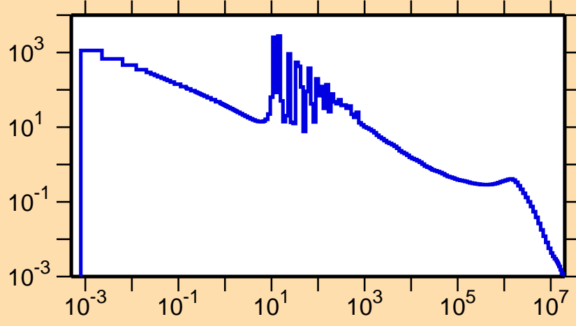
\sigma vs. E for ^{145}\text{Sm}(n,\gamma)
