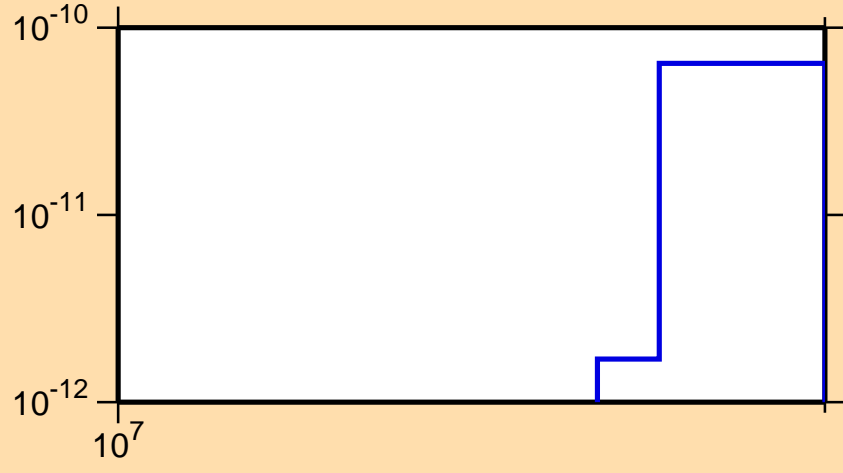
\sigma vs. E for ^{145}\text{Sm}(n,\text{pd})
