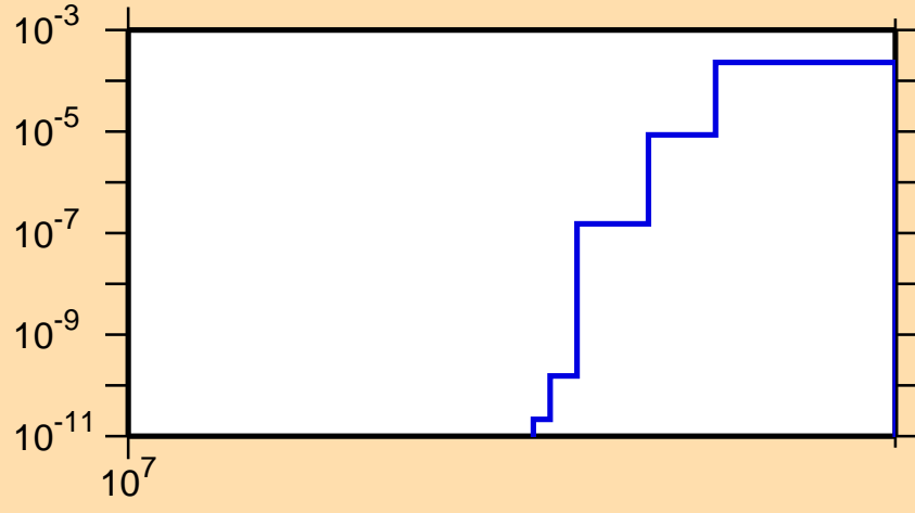
\sigma vs. E for ^{145}\text{Sm}(n,2np)
