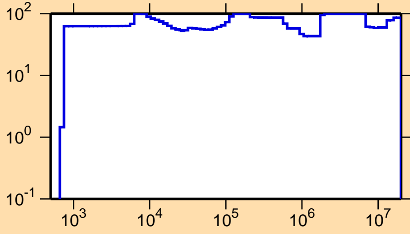
\Delta\sigma/\sigma vs. E for ^{145}\text{Sm}(n,p)
