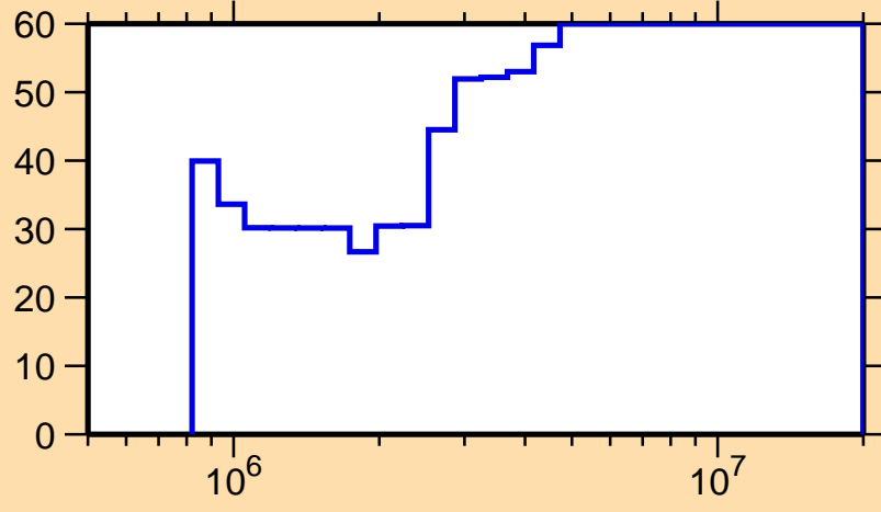
\Delta\sigma/\sigma vs. E for ^{145}\text{Sm}(n,n_1)
