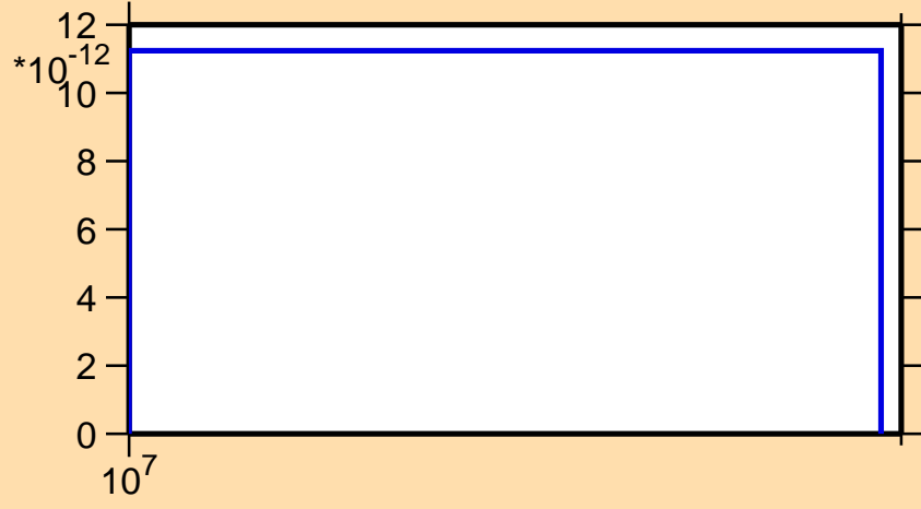
\sigma vs. E for ^{145}\text{Sm}(n,pt)
