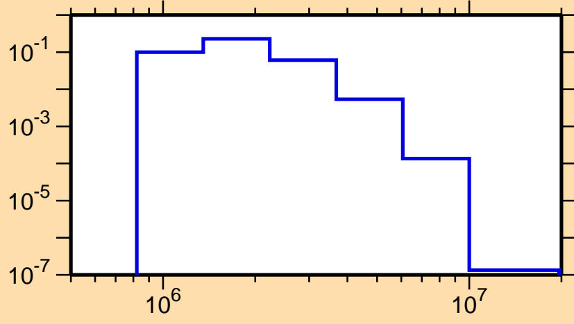
\sigma vs. E for ^{145}\text{Sm}(n,n_1)
