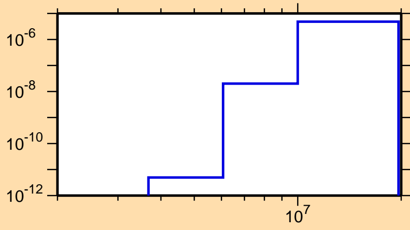
\sigma vs. E for ^{145}\text{Sm}(n,p\alpha)
