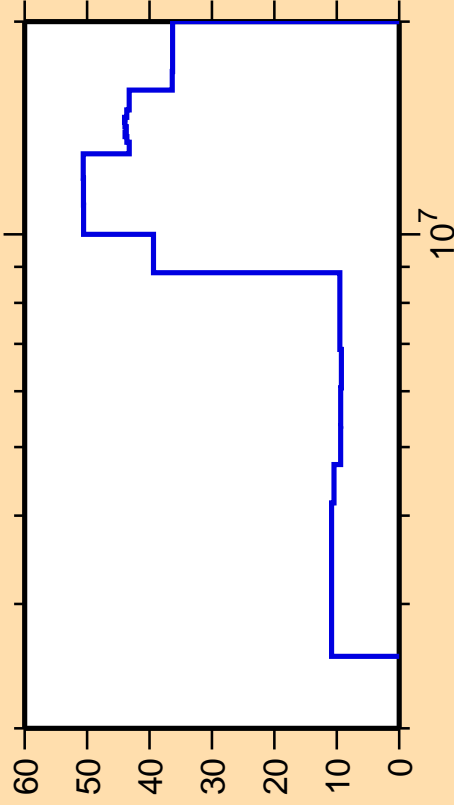
\Delta\sigma/\sigma vs. E for ^{146}\text{Sm}(n,n\text{cont.})
