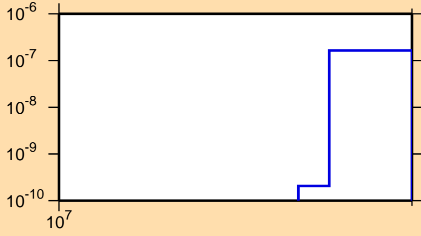
\sigma vs. E for ^{146}\text{Sm}(n,nt)
