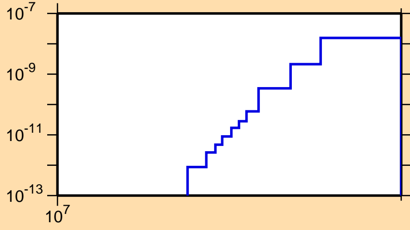
\sigma vs. E for ^{146}\text{Sm}(\text{mt117})
