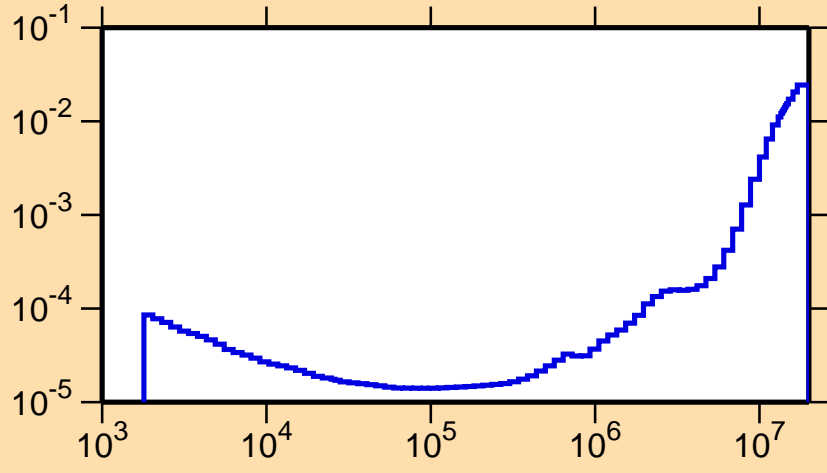
\sigma vs. E for ^{146}\text{Sm}(n,\alpha)
