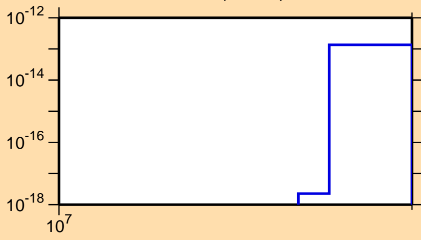
\sigma vs. E for ^{146}\text{Sm} (mt 34)
