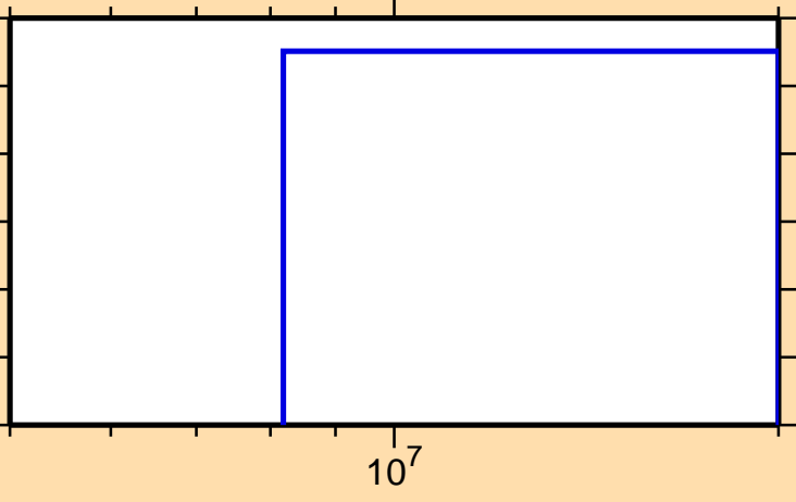
\sigma vs. E for ^{146}\text{Sm} (mt 34)
