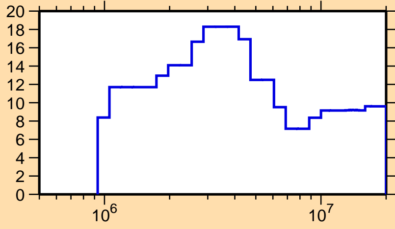
\Delta\sigma/\sigma vs. E for ^{147}\text{Sm}(n,el.)
