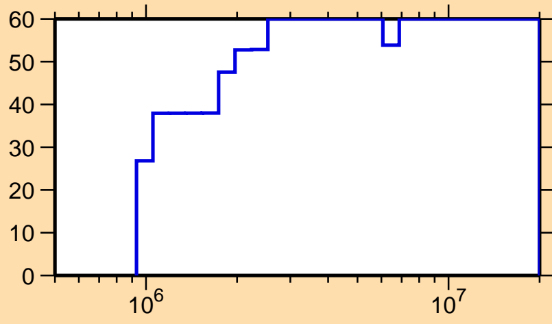
\Delta\sigma/\sigma vs. E for ^{147}\text{Sm}(n,\gamma)
