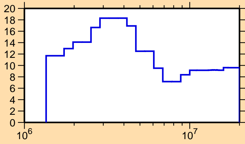
\Delta\sigma/\sigma vs. E for ^{147}\text{Sm}(n, el.)
