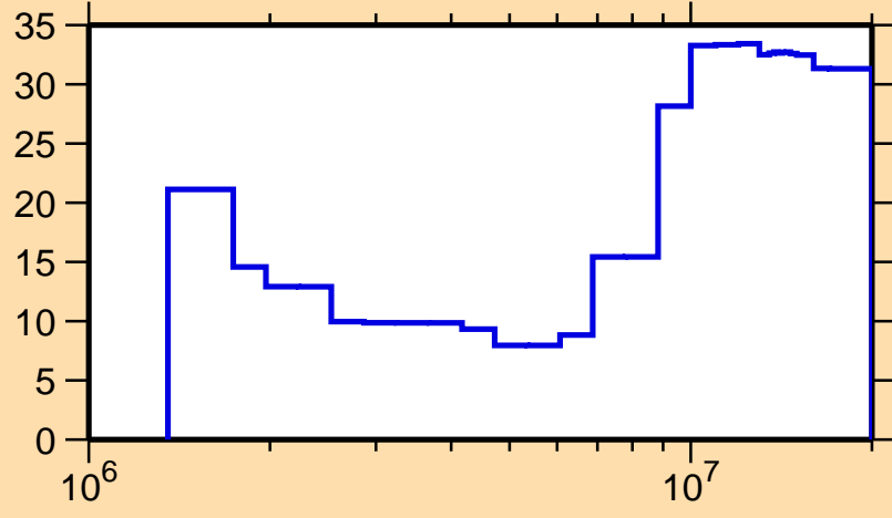
\Delta\sigma/\sigma vs. E for ^{147}\text{Sm}(n,n\text{cont.})
