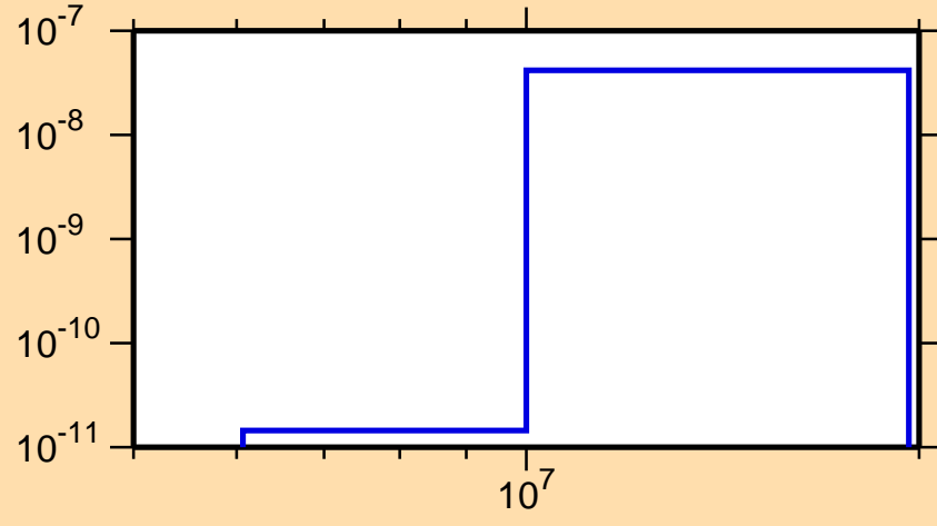
\sigma vs. E for ^{147}\text{Sm}(n,p\alpha)
