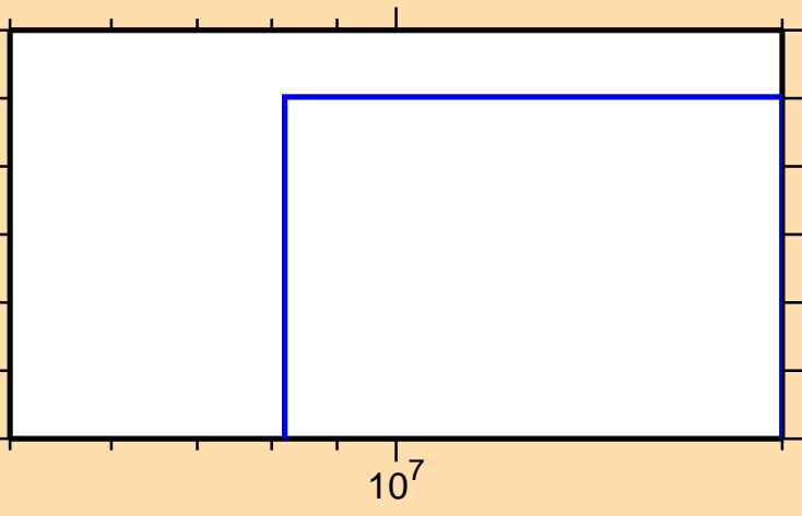
\sigma vs. E for ^{147}\text{Sm}(n,\text{He}3)
