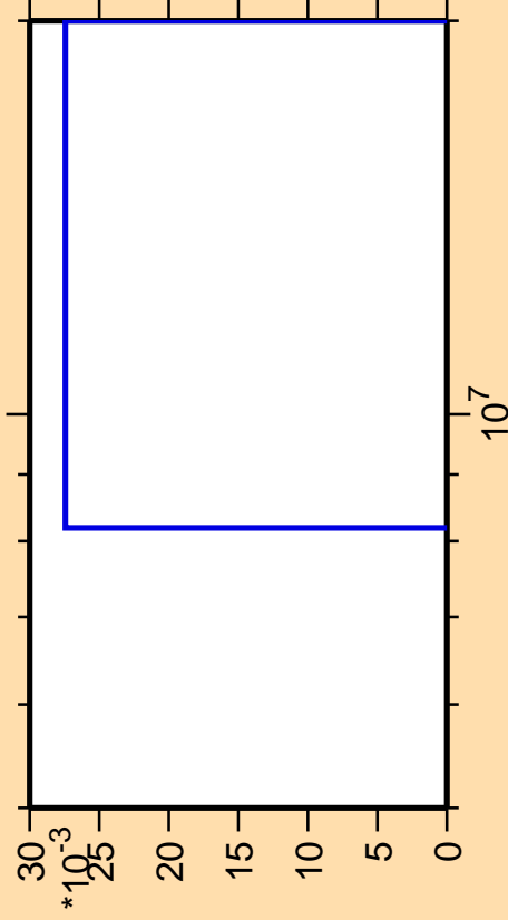
\Delta\sigma/\sigma vs. E for ^{147}\text{Sm}(n,3n\alpha)
