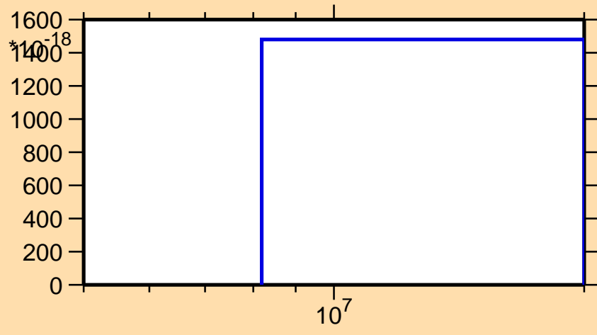
\sigma vs. E for ^{147}\text{Sm}(n,\text{pd})
