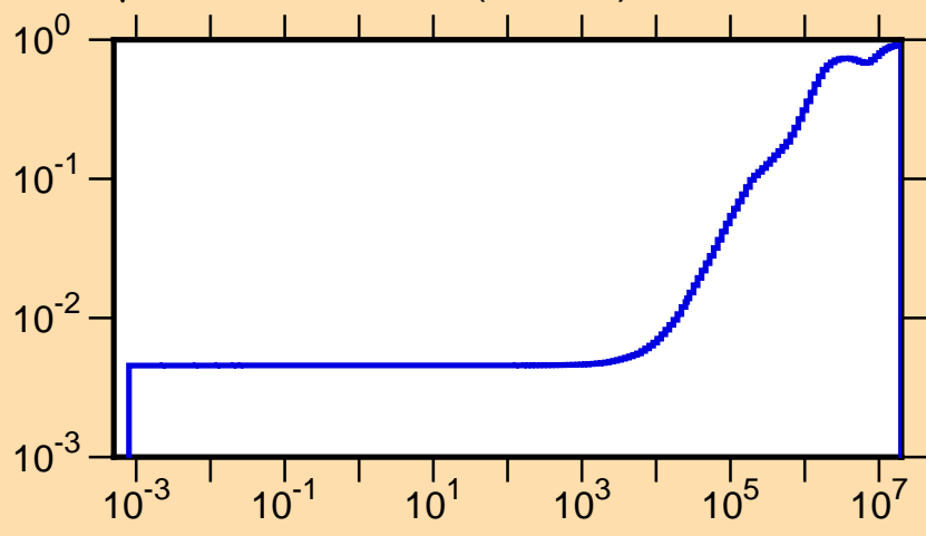
\mu vs. E for ^{148}\text{Sm}(\text{mt251})
