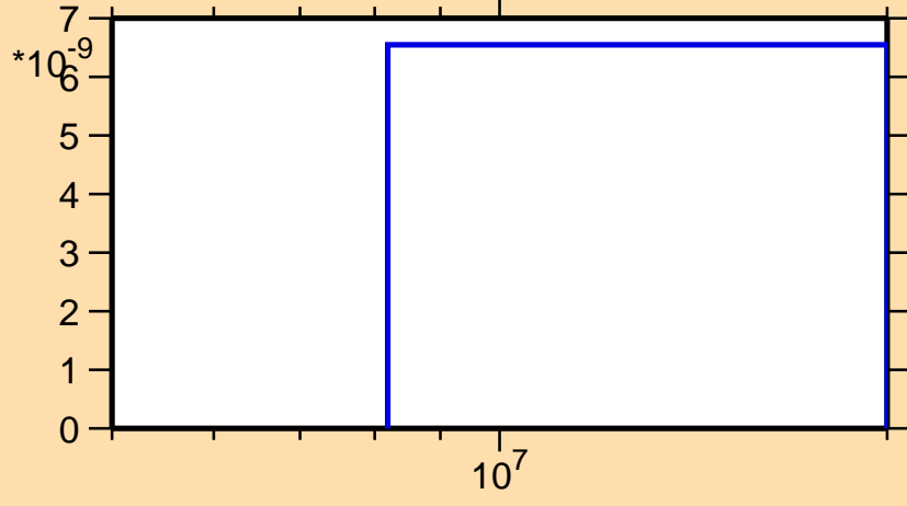
\sigma vs. E for ^{148}\text{Sm}(n,nd)
