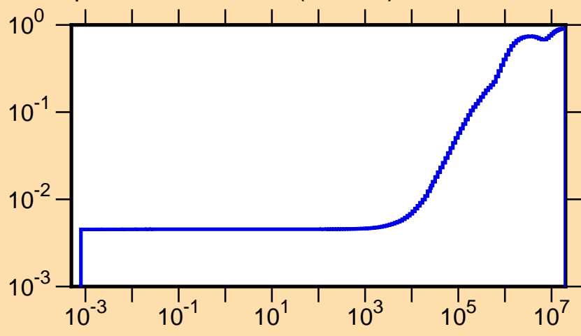
\mu vs. E for ^{149}\text{Sm}(\text{mt251})
