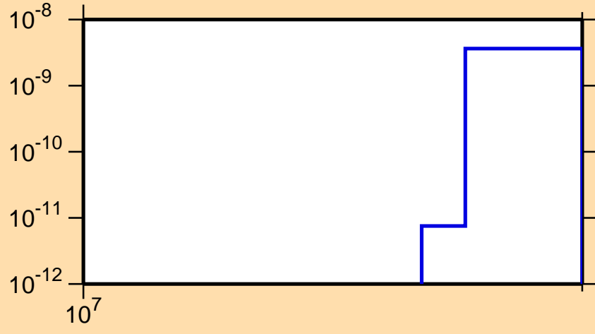
\sigma vs. E for ^{149}\text{Sm}(n,3n\alpha)
