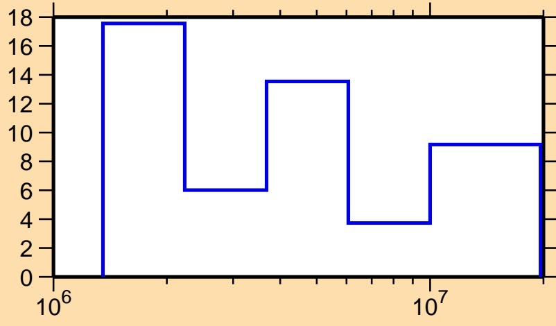
\Delta\sigma/\sigma vs. E for ^{149}\text{Sm}(n,el.)
