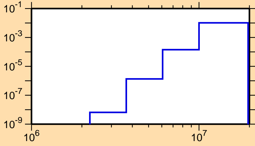
\sigma vs. E for ^{149}\text{Sm}(n,p)
