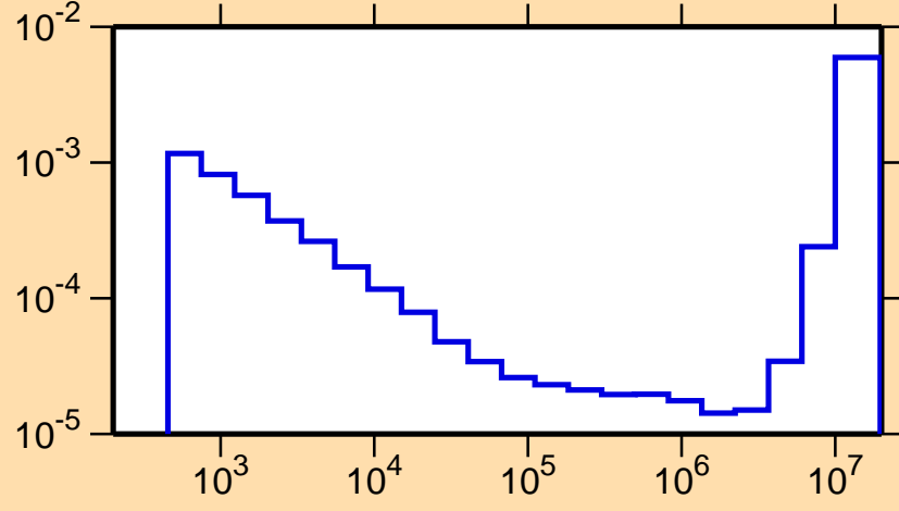
\sigma vs. E for ^{149}\text{Sm}(n,\alpha)
