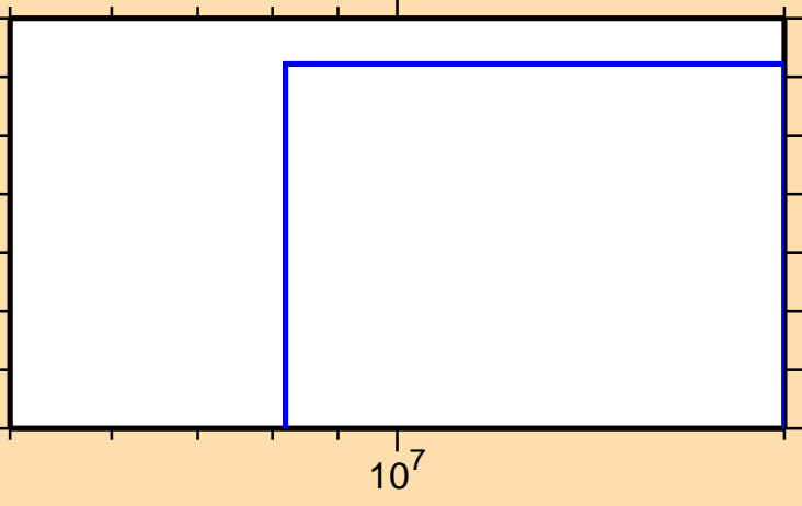
\sigma vs. E for ^{149}\text{Sm}(n,\text{nd})
