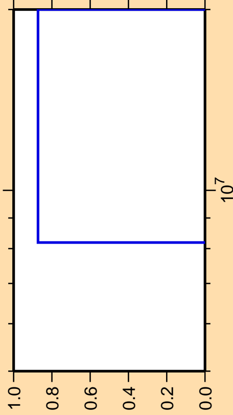
\Delta\sigma/\sigma vs. E for ^{149}\text{Sm} (mt 45)
