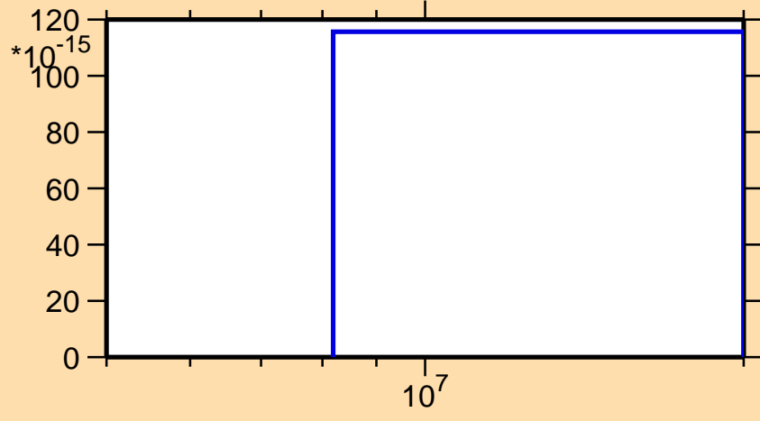
\sigma vs. E for ^{149}\text{Sm} (mt 45)
