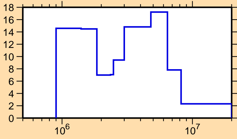
\Delta\sigma/\sigma vs. E for ^{149}\text{Sm}(n,\text{tot.})
