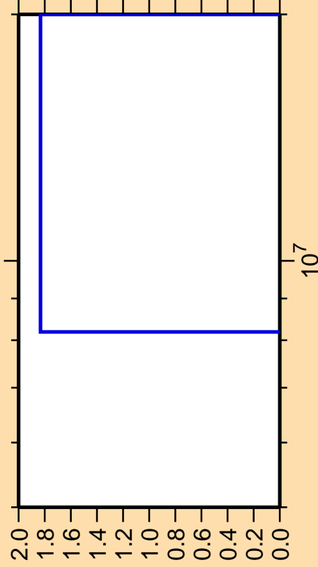
\Delta\sigma/\sigma vs. E for ^{149}\text{Sm}(\text{mt117})
