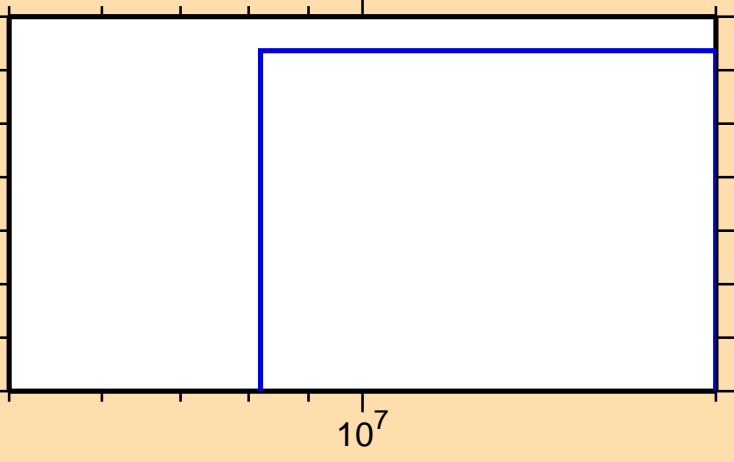
\sigma vs. E for ^{149}\text{Sm} (mt 34)
