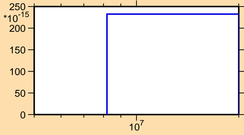
\sigma vs. E for ^{149}\text{Sm}(\text{mt117})
