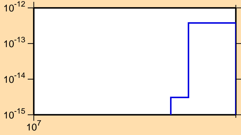
\sigma vs. E for ^{150}\text{Sm} (mt 45)
