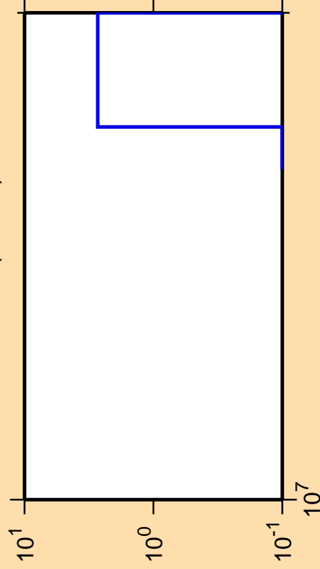
\Delta\sigma/\sigma vs. E for ^{150}\text{Sm} (mt 45)
