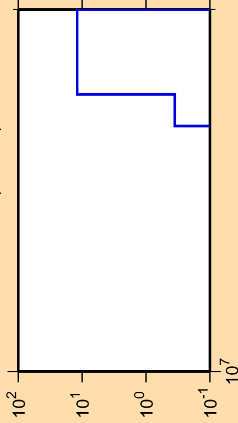
\Delta\sigma/\sigma vs. E for ^{150}\text{Sm}(\text{mt117})
