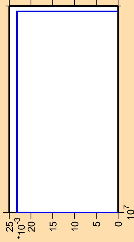
\Delta\sigma/\sigma vs. E for ^{150}\text{Sm} (mt 45)
