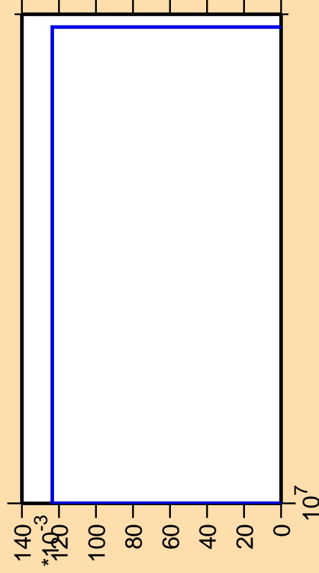
\Delta\sigma/\sigma vs. E for ^{150}\text{Sm}(\text{mt117})
