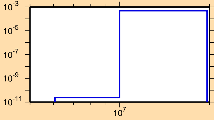
\sigma vs. E for ^{150}\text{Sm}(n,d)
