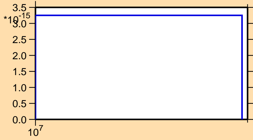
\sigma vs. E for ^{150}\text{Sm} (mt 45)
