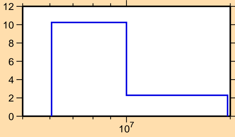
\Delta\sigma/\sigma vs. E for ^{150}\text{Sm}(n,\text{tot.})
