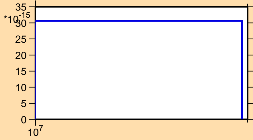
\sigma vs. E for ^{150}\text{Sm}(\text{mt117})
