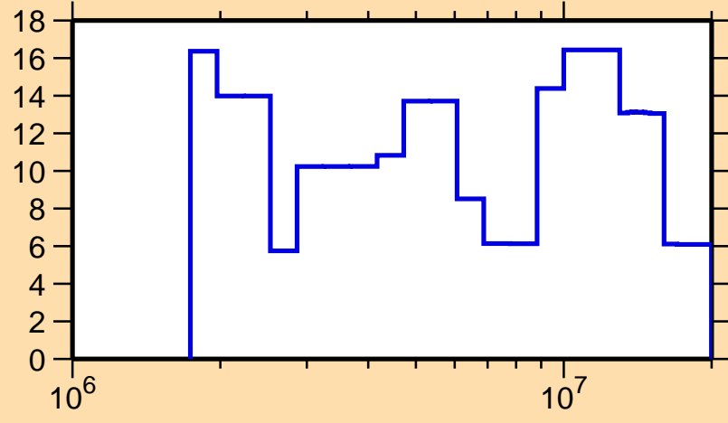
\Delta\sigma/\sigma vs. E for ^{151}\text{Sm}(n,el.)
