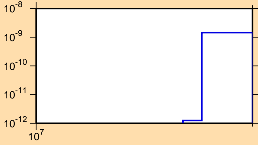
\sigma vs. E for ^{151}\text{Sm}(n,3n\alpha)
