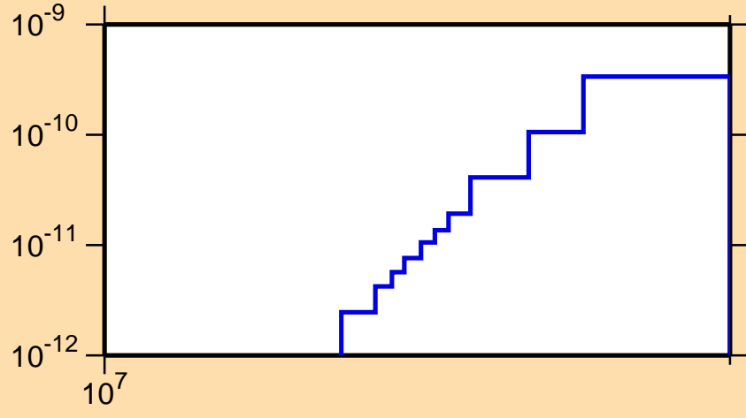
\sigma vs. E for ^{151}\text{Sm}(n,p\alpha)
