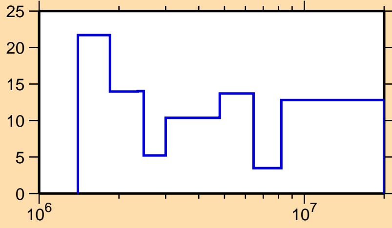
\Delta\sigma/\sigma vs. E for ^{151}\text{Sm}(n,el.)
