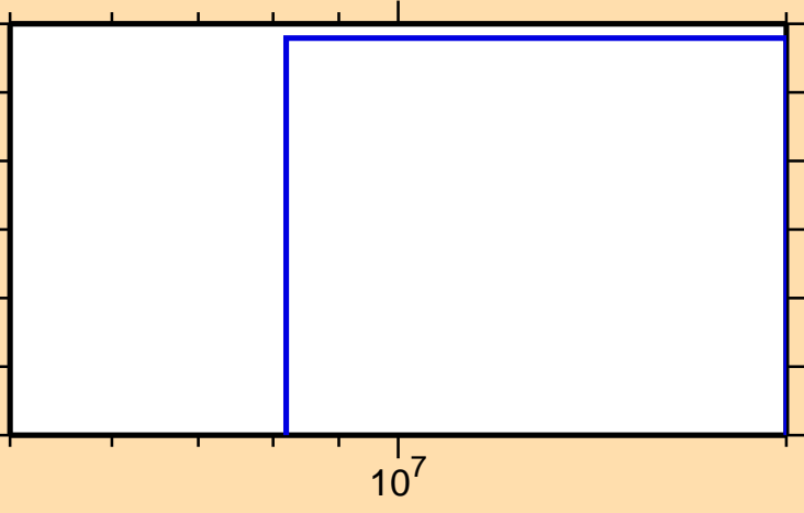
\sigma vs. E for ^{151}\text{Sm}(n,3n)
