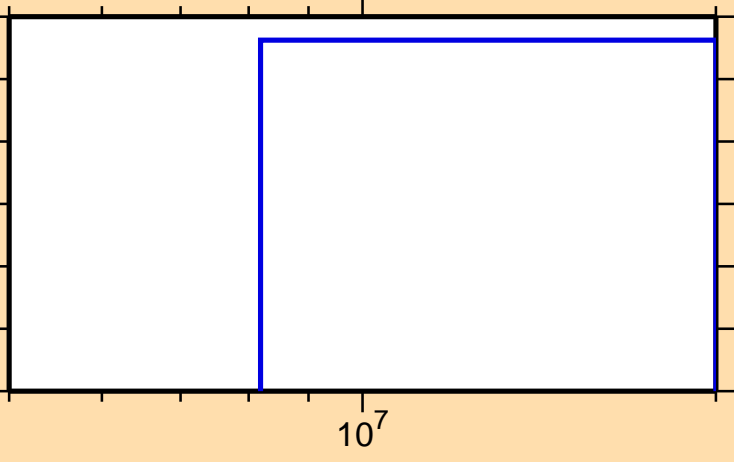
\sigma vs. E for ^{151}\text{Sm}(n,\text{nd})
