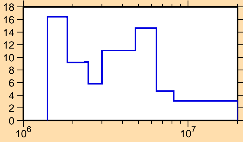
\Delta\sigma/\sigma vs. E for ^{151}\text{Sm}(n,\text{tot.})
