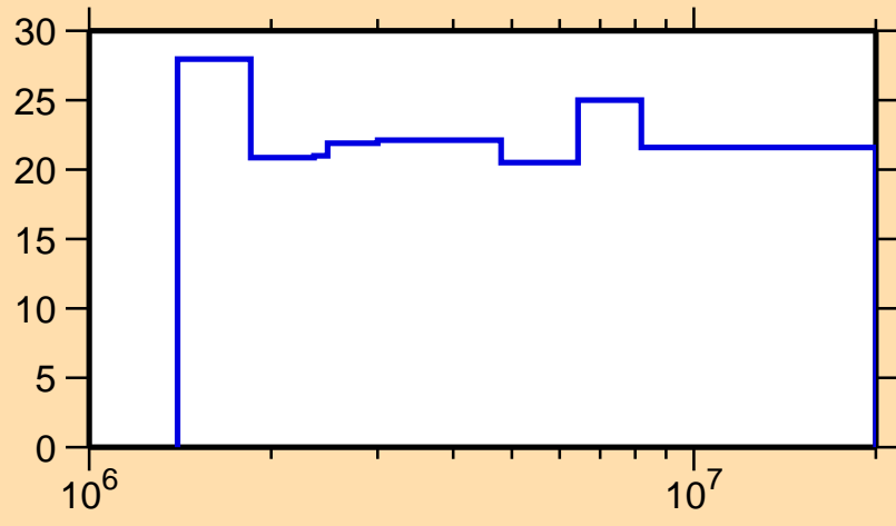
\Delta\sigma/\sigma vs. E for ^{151}\text{Sm}(n,ncont.)
