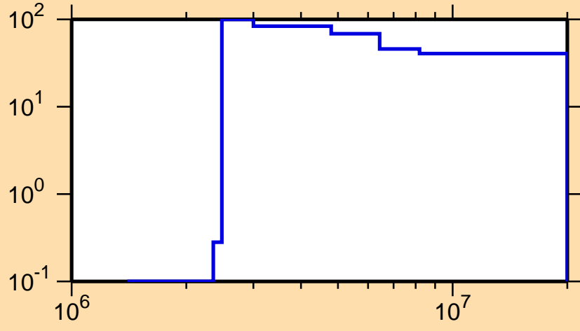
\Delta\sigma/\sigma vs. E for ^{151}\text{Sm}(n,p)
