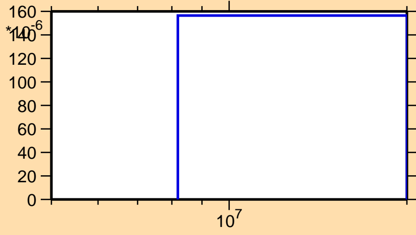
\sigma vs. E for ^{151}\text{Sm}(n,np)
