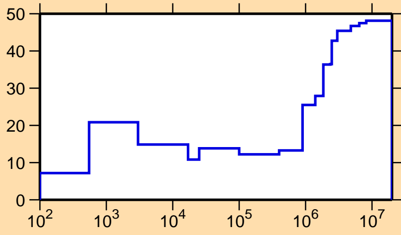
\Delta\sigma/\sigma vs. E for ^{151}\text{Sm}(n,\gamma)
