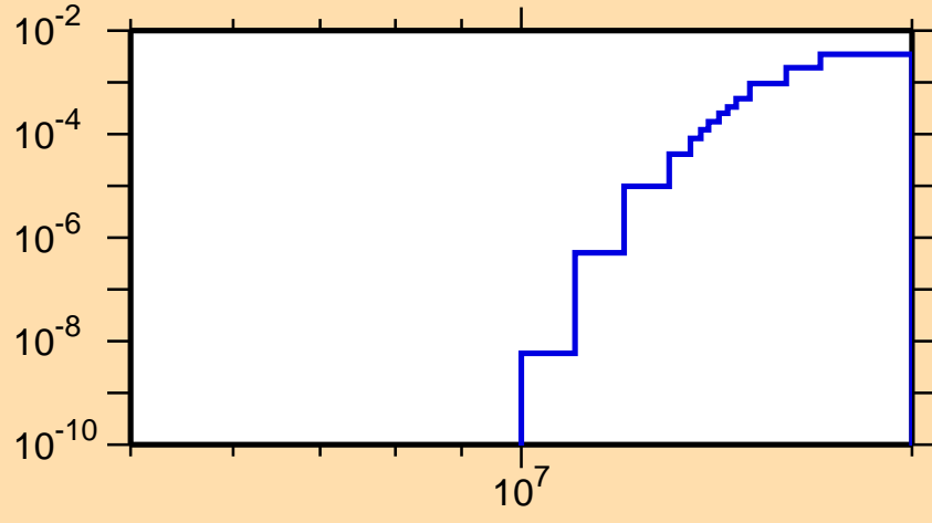
\sigma vs. E for ^{152}\text{Sm}(n,d)
