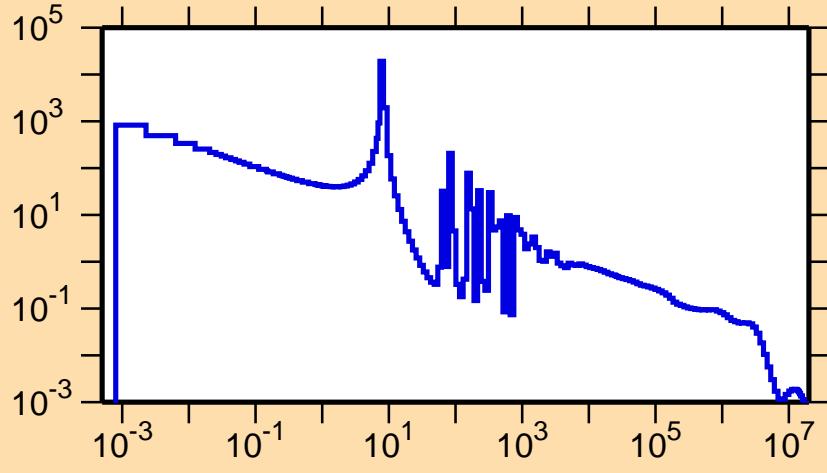
\sigma vs. E for ^{152}\text{Sm}(n,\gamma)
