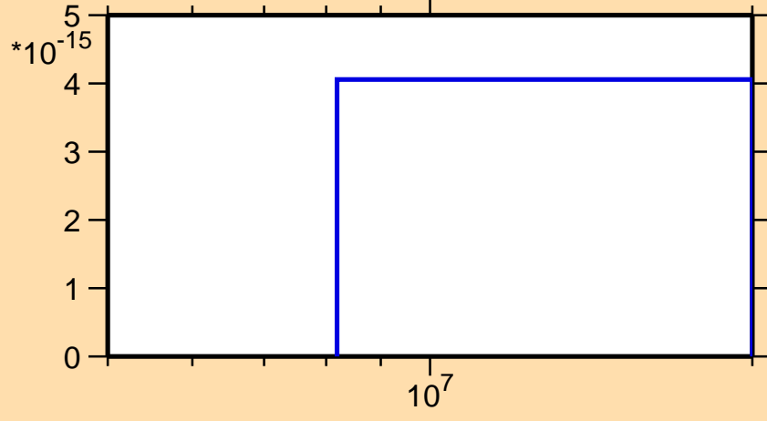
\sigma vs. E for ^{152}\text{Sm}(n,p\alpha)
