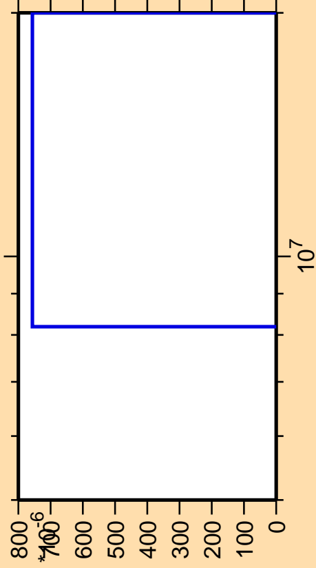
\Delta\sigma/\sigma vs. E for ^{152}\text{Sm}(n,p\alpha)
