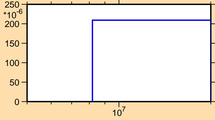
\sigma vs. E for ^{152}\text{Sm}(n,np)
