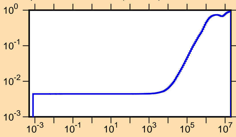
\mu vs. E for ^{153}\text{Sm}(\text{mt251})
