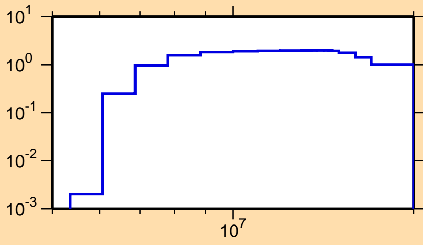
\sigma vs. E for ^{153}\text{Sm}(n,2n)
