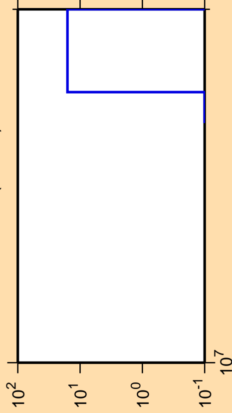
\Delta\sigma/\sigma vs. E for ^{153}\text{Sm}(n,3n\alpha)
