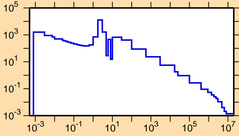
\sigma vs. E for ^{153}\text{Sm}(n,\gamma)
