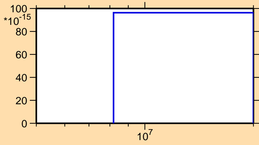
\sigma vs. E for ^{153}\text{Sm}(n,\text{He3})
