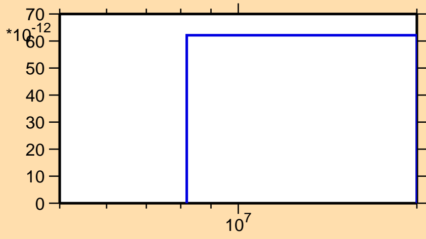
\sigma vs. E for ^{153}\text{Sm}(n,nt)
