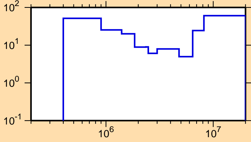
\Delta\sigma/\sigma vs. E for ^{153}\text{Sm}(n,n\text{cont.})
