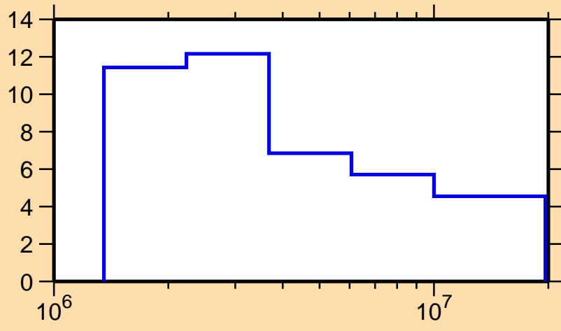
\Delta\sigma/\sigma vs. E for ^{154}\text{Sm}(n, el.)
