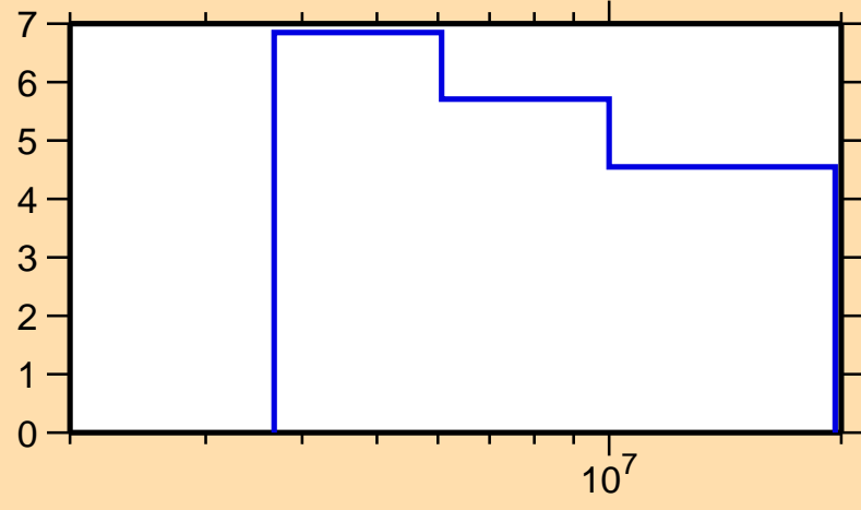
\Delta\sigma/\sigma vs. E for ^{154}\text{Sm}(n,el.)
