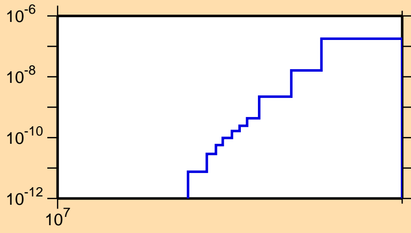
\sigma vs. E for ^{155}\text{Sm}(n,2n\alpha)
