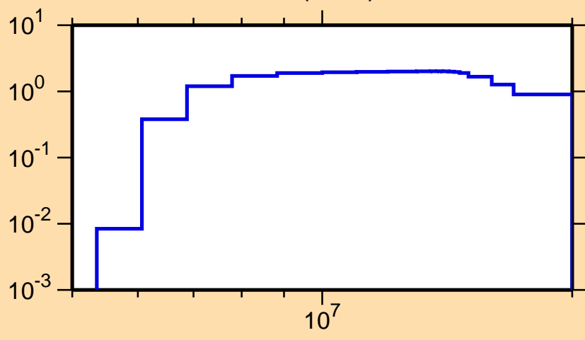
\sigma vs. E for ^{155}\text{Sm}(n,2n)
